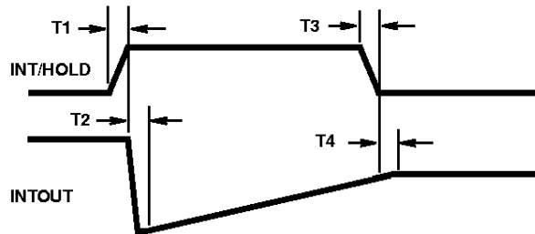
FIGURE 8. INTEGRATOR TIMING
