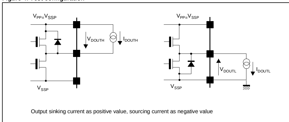
Figure 4. Test configuration
