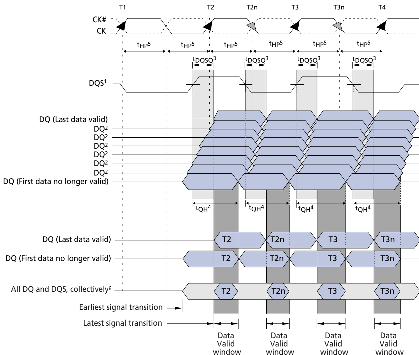
Figure 39: x4, x8 Data Output Timing – t_{DQSQ} , t_{QH} , and Data Valid Window
