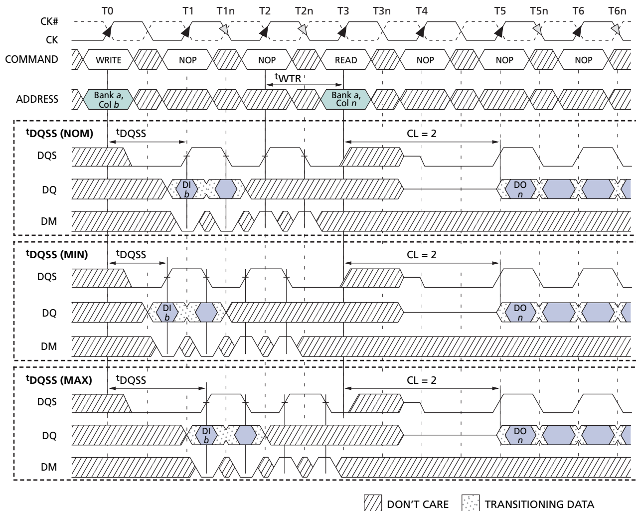
Figure 25: WRITE to READ - Interrupting
