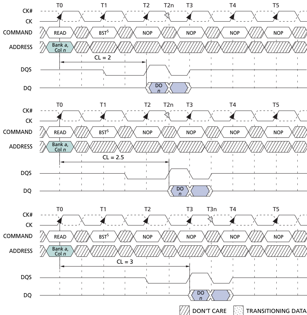
Figure 16: Terminating a READ Burst
