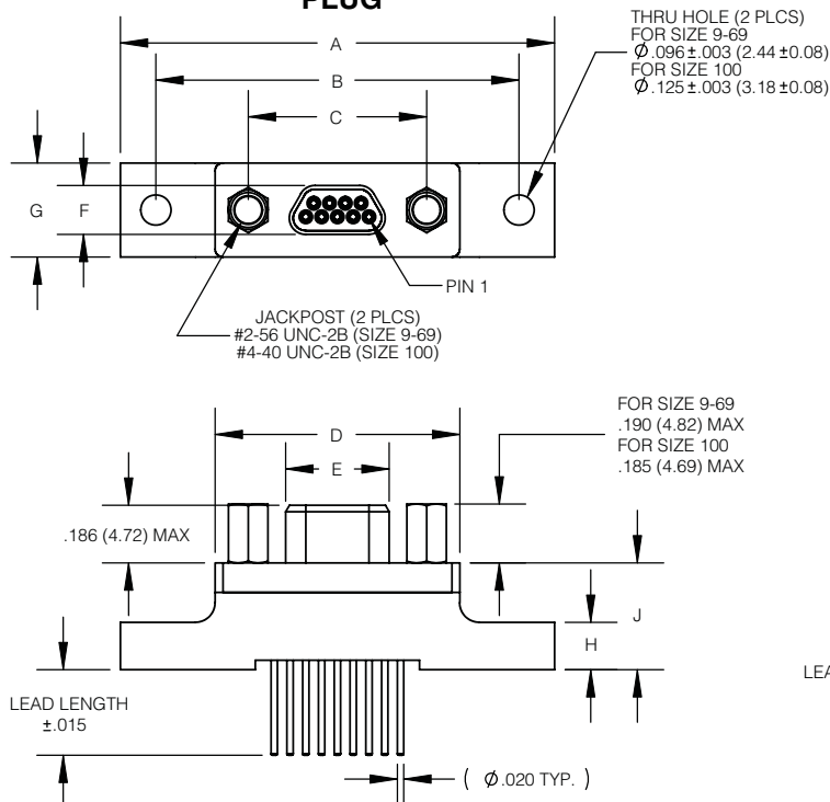
PLUG
