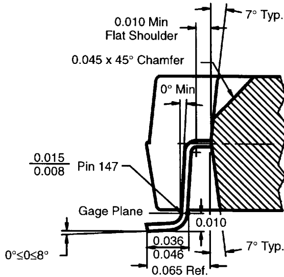
Detail X
