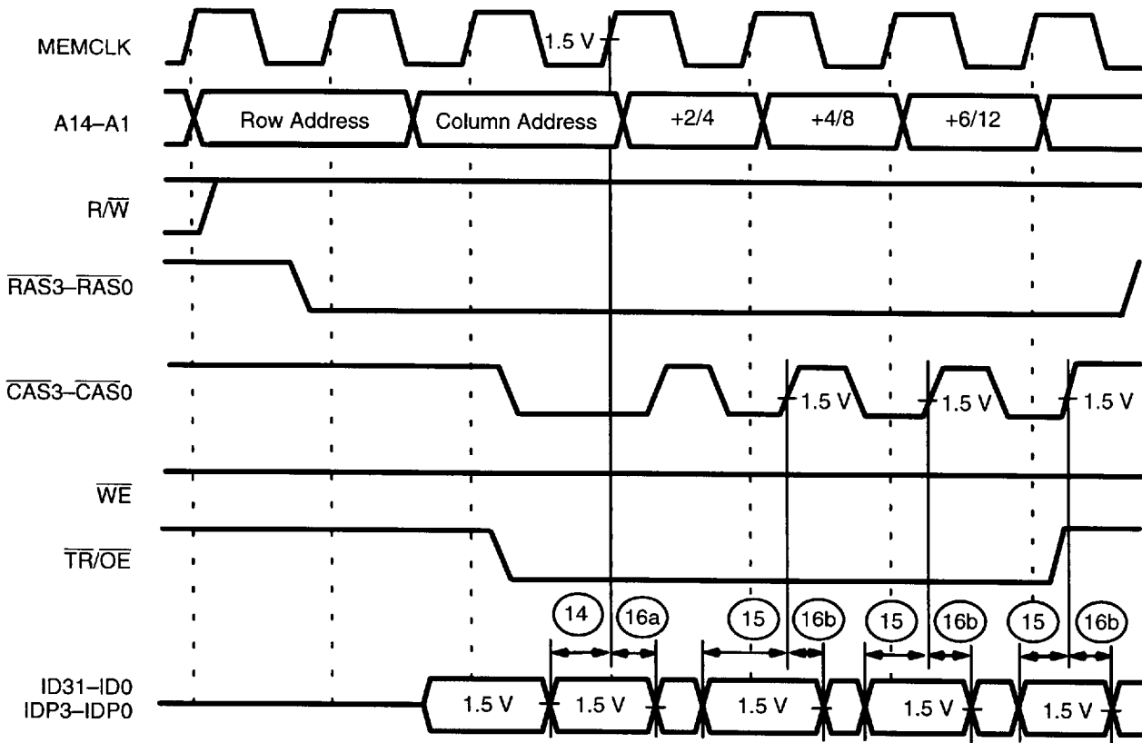
Figure 3. 3/1 DRAM Page-Mode Read, Am29240 Microcontroller Series
