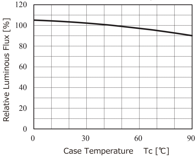
Case Temperature vs. Relative Luminous Flux I F = 950mA
