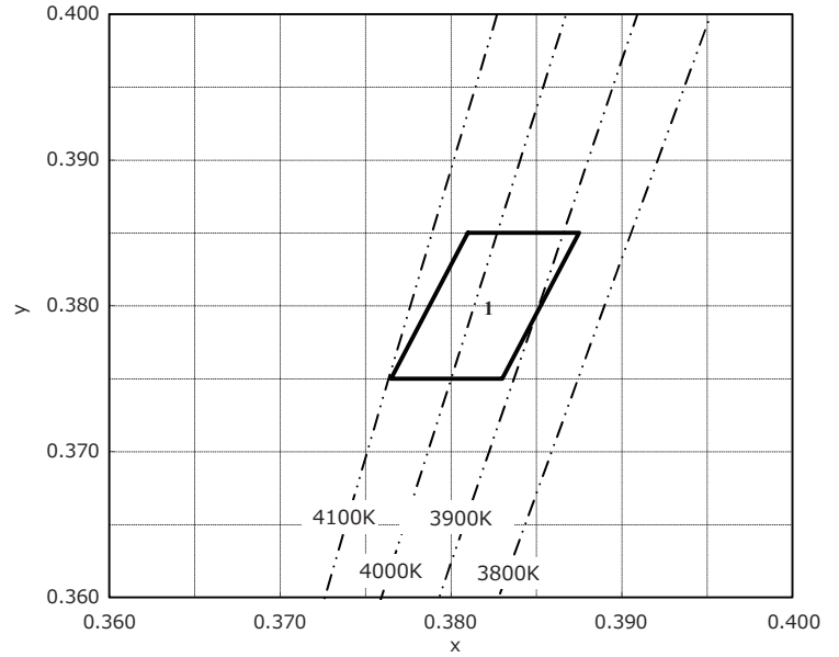
4 000K Chromaticity Diagram
