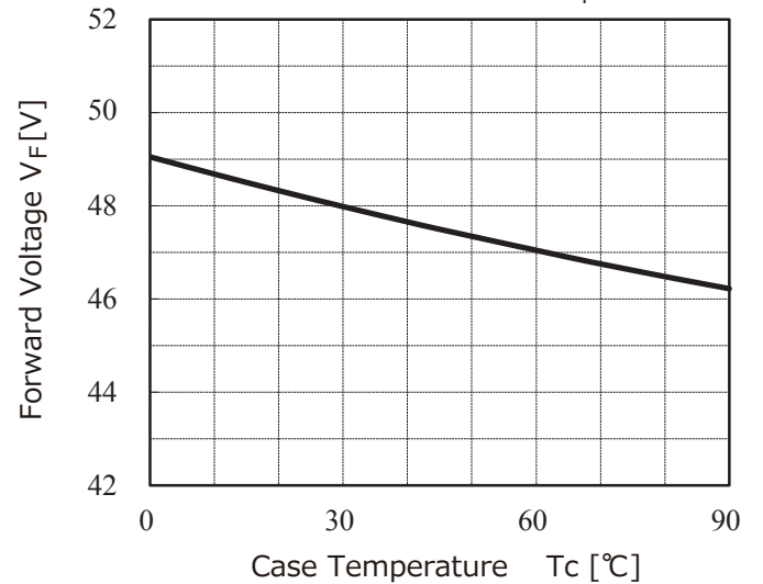
Case Temperature vs.Forward Voltage I F = 950mA
