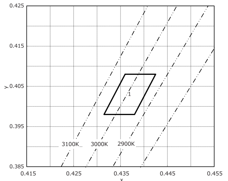
3 000K Chromaticity Diagram
