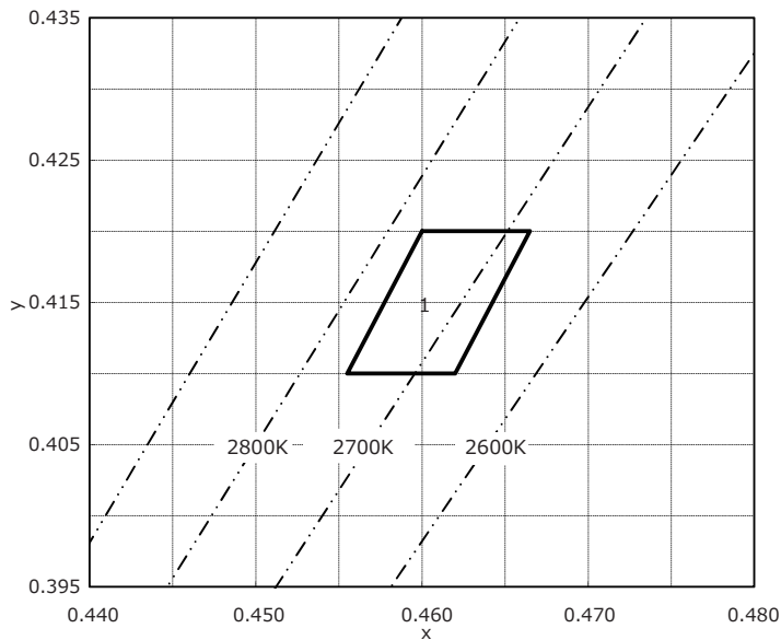
2 700K Chromaticity Diagram
