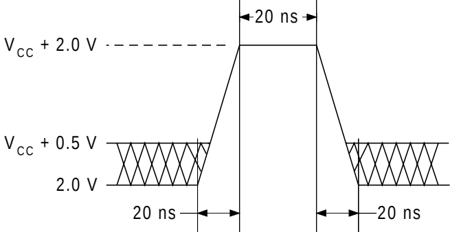
Figure 10. Maximum Overshoot Waveform
