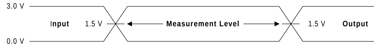
HY29F400-45 Version
