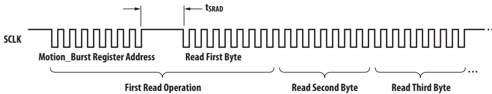
Figure 20. Motion Burst Timing
