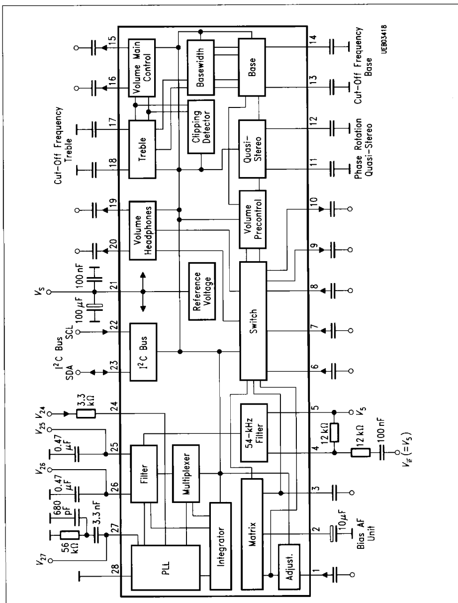
Test Circuit 2
