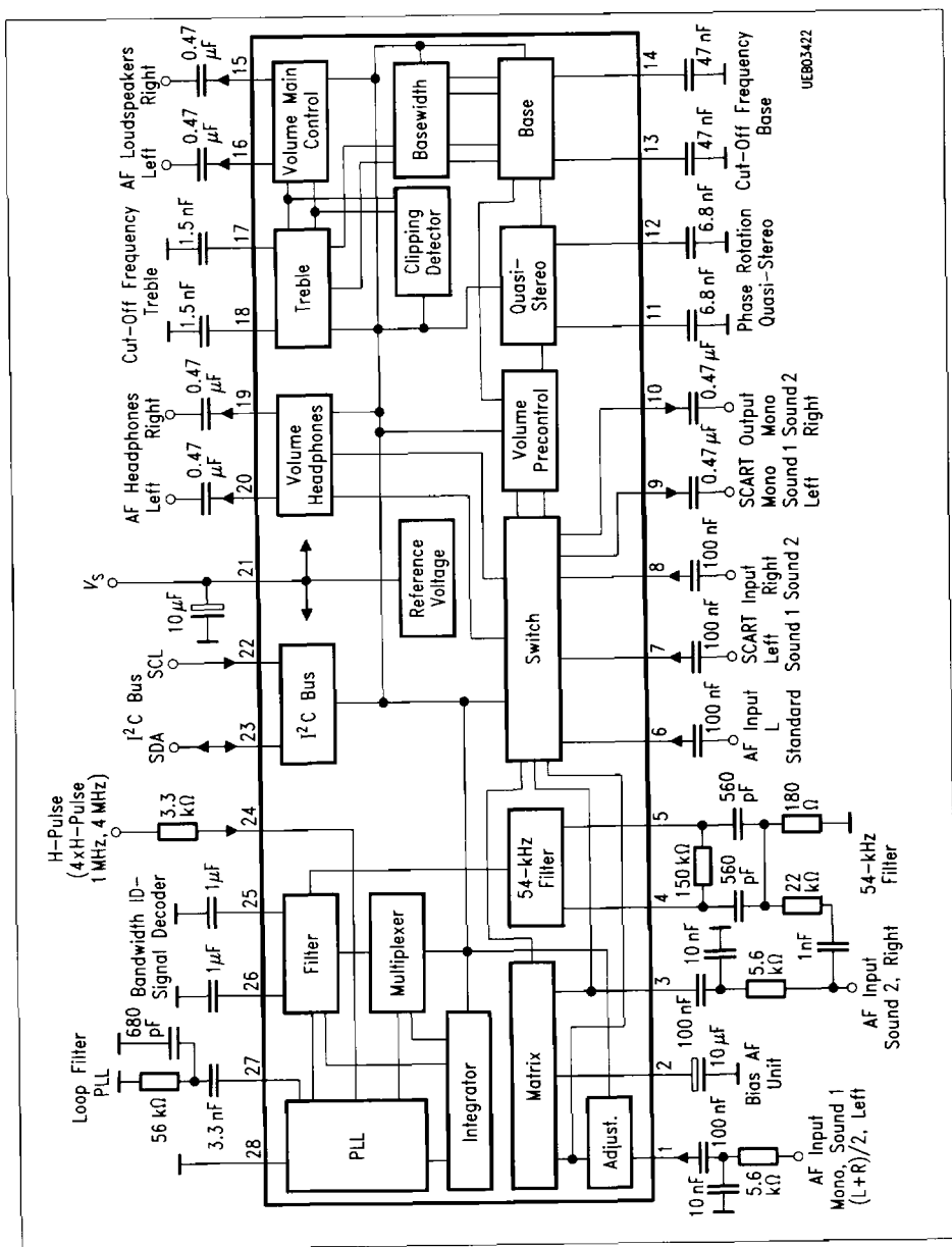
Application Circuit 2
