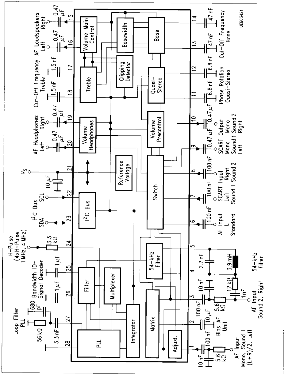
Application Circuit 1
