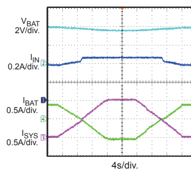
Power Path Management MODE=0, W/ Battery
