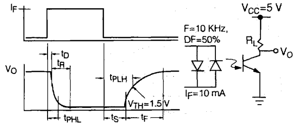
Figure 14. Switching timing and schematic
