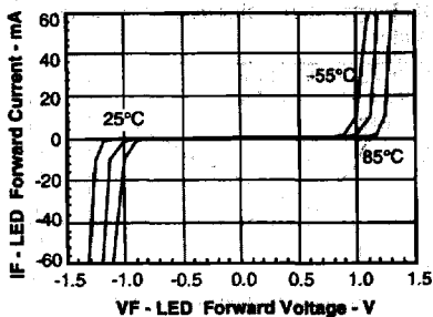
Figure 1. LED forward current versus forward voltage
