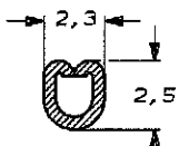
SECTION A-A ENLARGED VIEW
