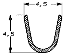
SECTION B-B ENLARGED VIEW
