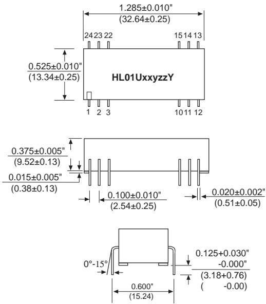
DIP PACKAGE
