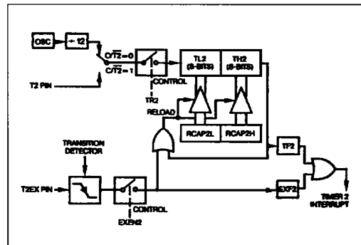
Figure 3 : Timer in Auto-Reload Mode.
