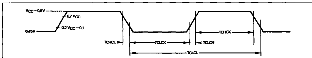
Figure 13 : Clock Signal Waveform for ICC Tests in Active and Idle Modes. TCHL = TCHX = 5 ns.
