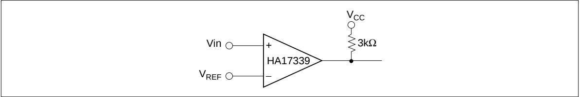
Figure 6 Basic Comparator
