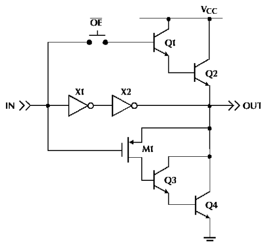
Figure 6. One Buffer Cell of the ML65F16245
