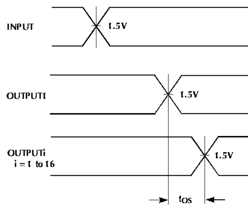
Figure 10. Output Skew
