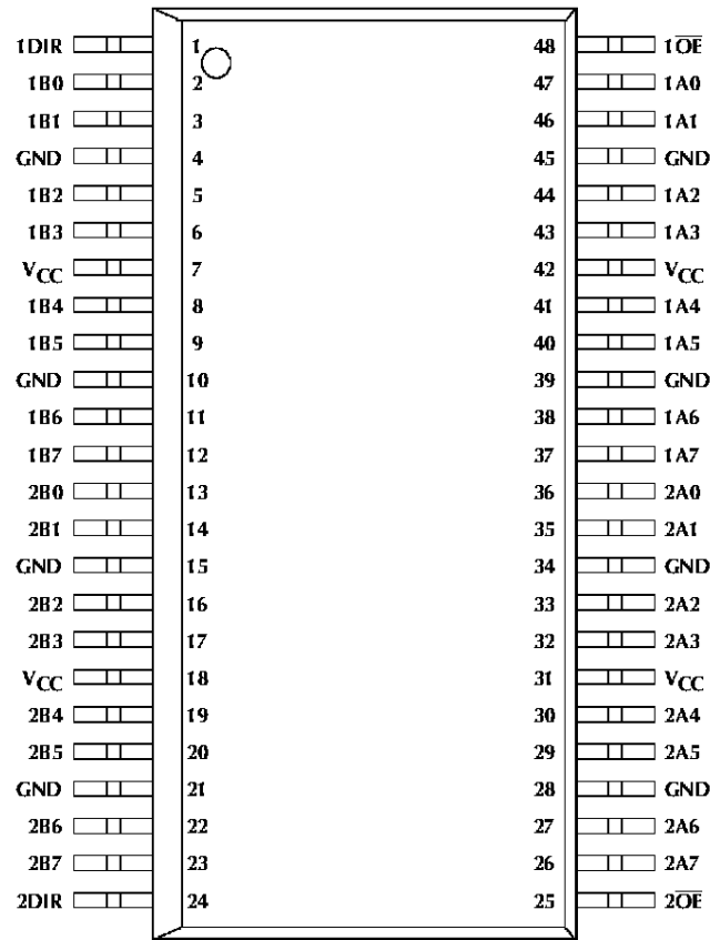
TOP VIEW
