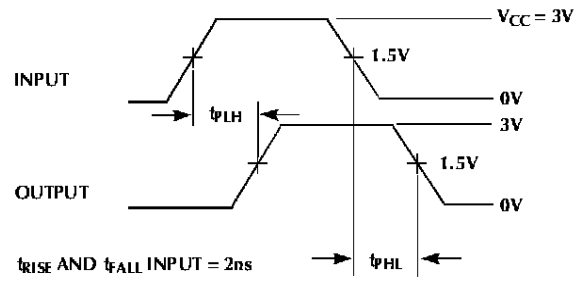
Figure 8. Propagation Delay
