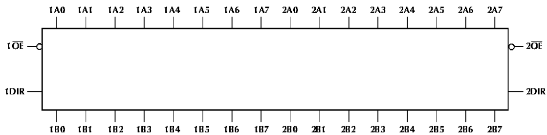
Figure 5. Logic Symbol
