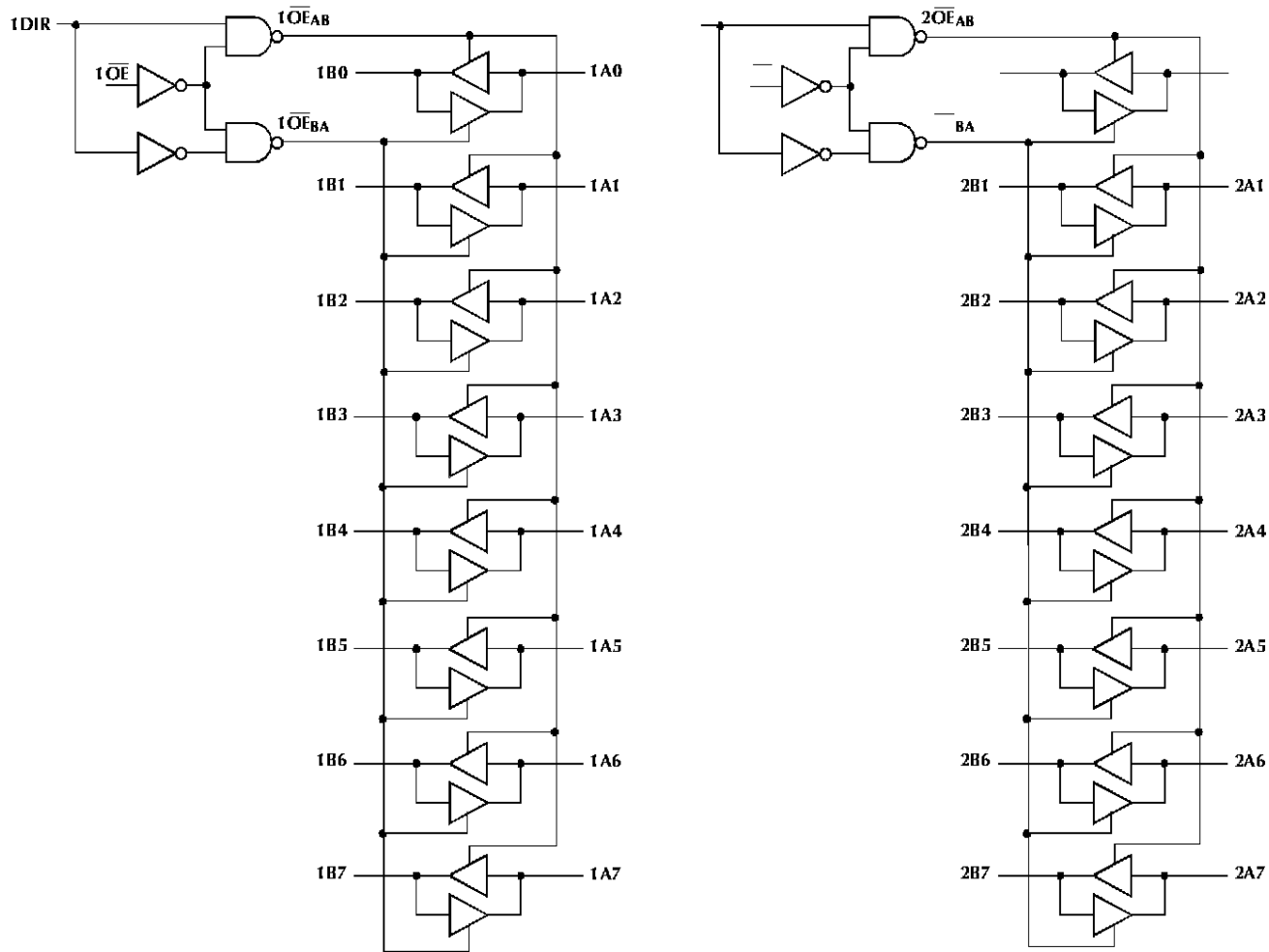
Figure 4. Logic Diagram
