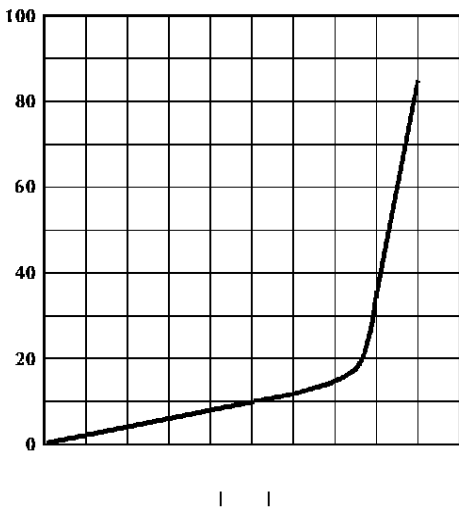
Figure 1a. Typical V_{OL} vs. I_{OL} for 3.3V V_{CC} . One Buffer Output
