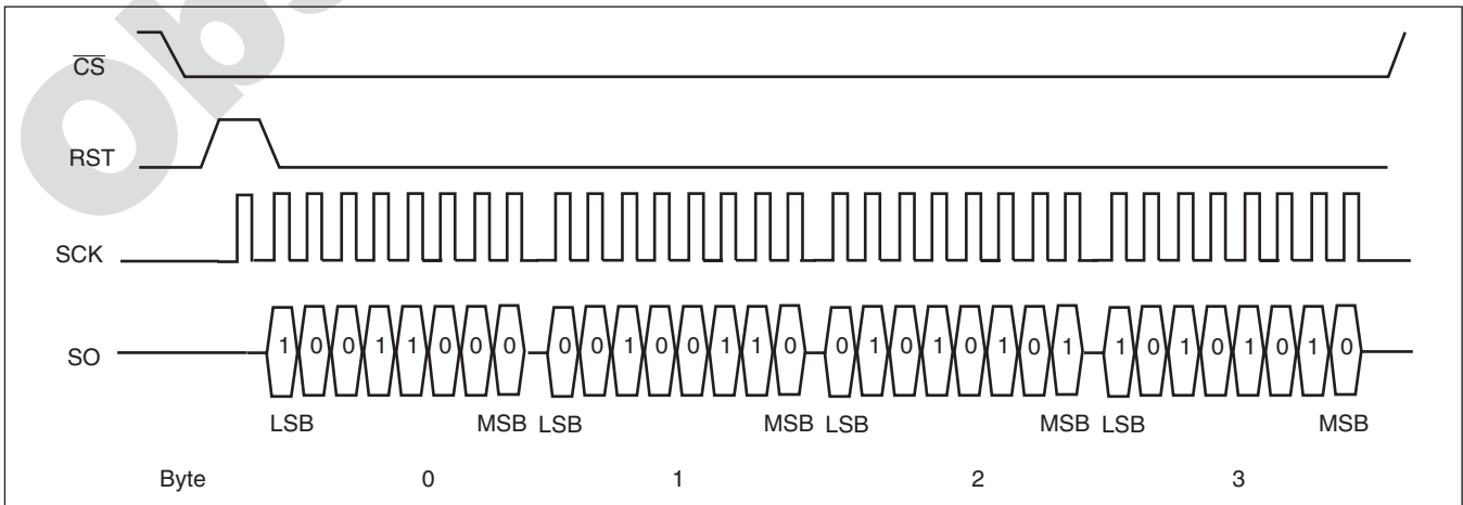
Figure 11. Response to RESET(RST)
