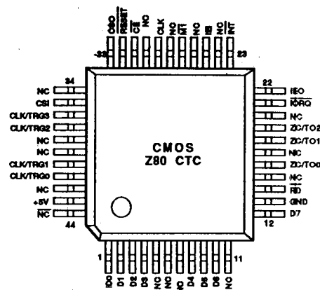
Figure 2C. 44-Pin LQFP Pin Assignments
