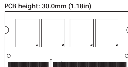
Figure 1: 204-Pin SODIMM (MO-268 R/C D)
