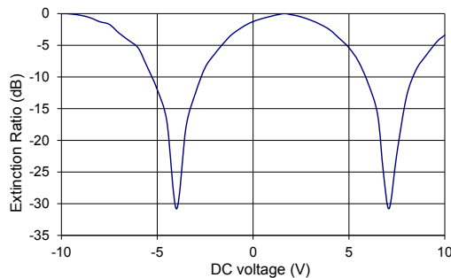
Extinction Ratio
