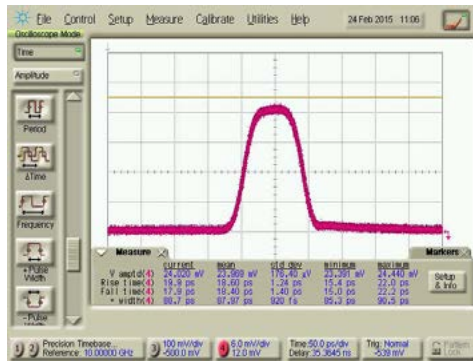
Extinction Ratio
