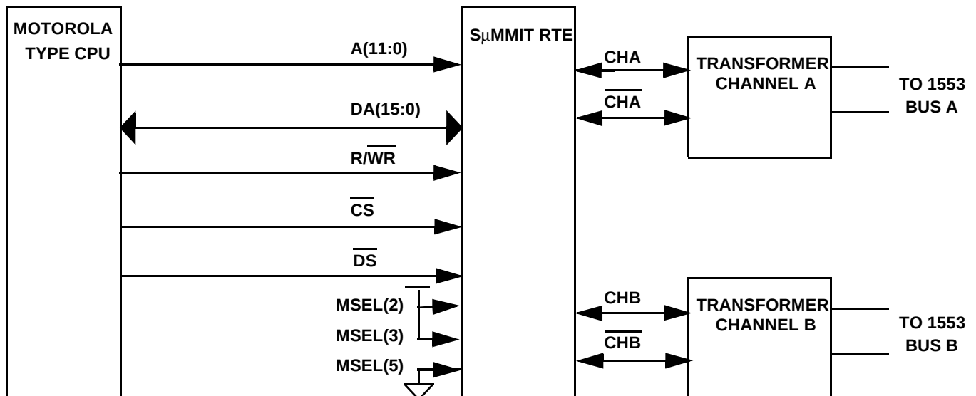
Figure 13b. 16-bit Interface (Motorola Type)
