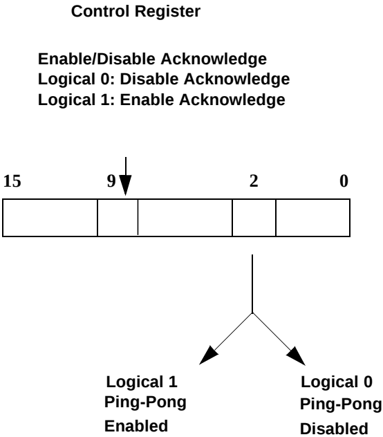
Figure 7. Ping-Pong Handshake
