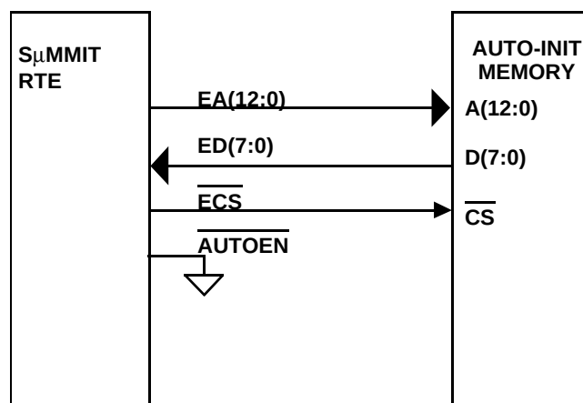
Figure 11a. Auto-Initialization System Configuration
