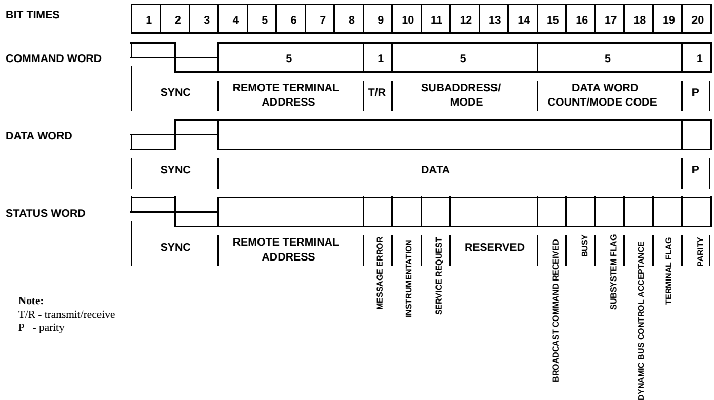
Figure 16. MIL-STD-1553B Word Formats
