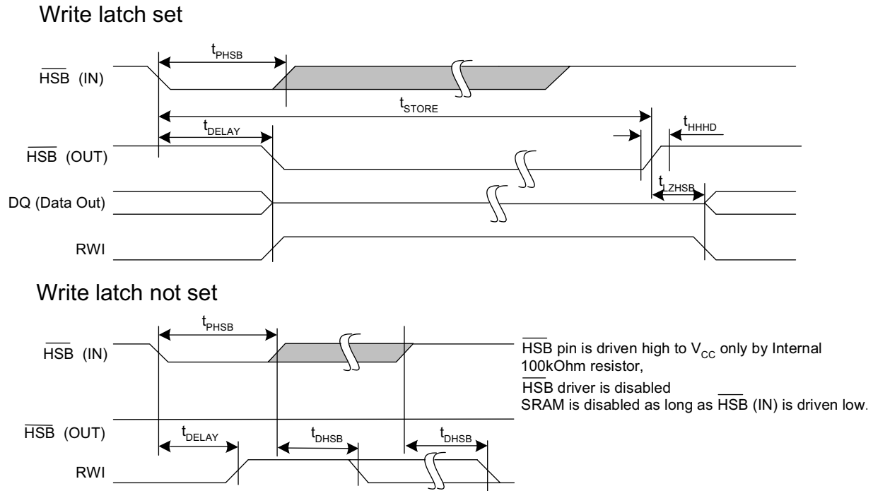
Figure 13. Hardware STORE Cycle [17]
