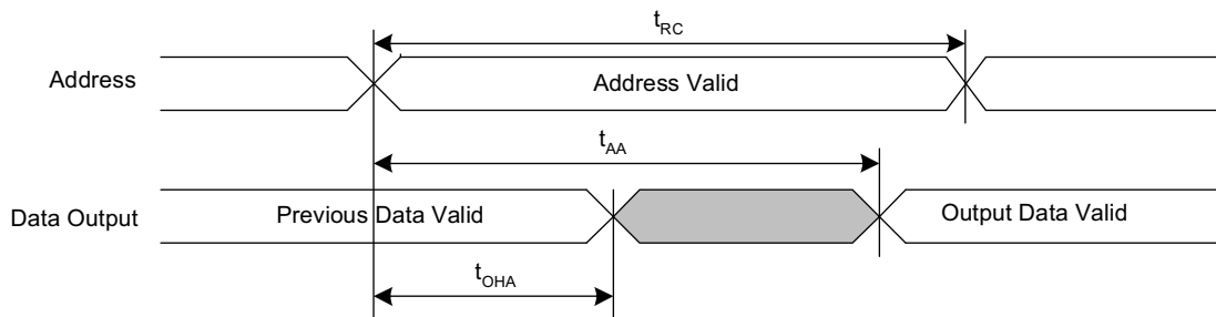
Figure 5. SRAM Read Cycle #1: Address Controlled [10, 11, 14]
