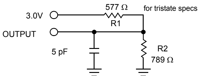
Figure 4. AC Test Loads
