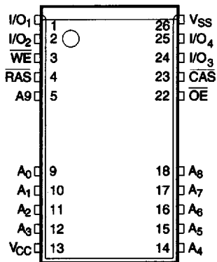
26/20-pin SOJ ( 300mil ) P26/20SJ-2A
