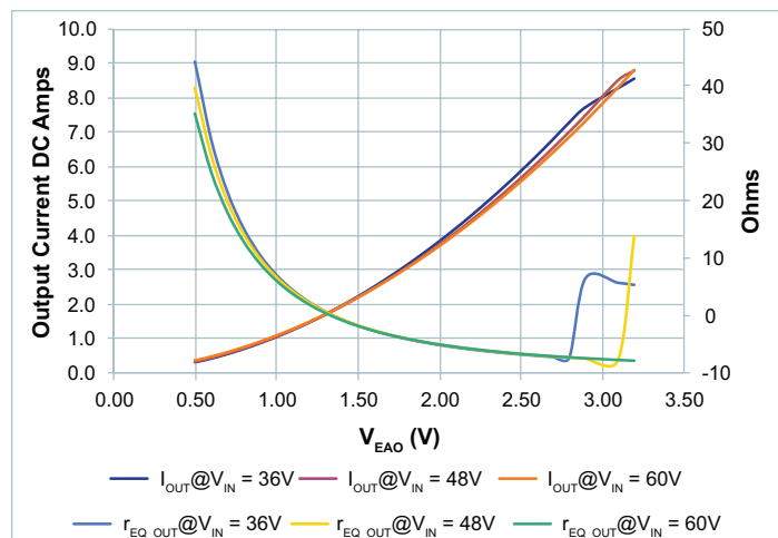
Figure 74 — r_{EQ\_OUT} vs. output current vs. V_{EAO} , V_{OUT} = 12V ; 36 – 60 V_{IN}
