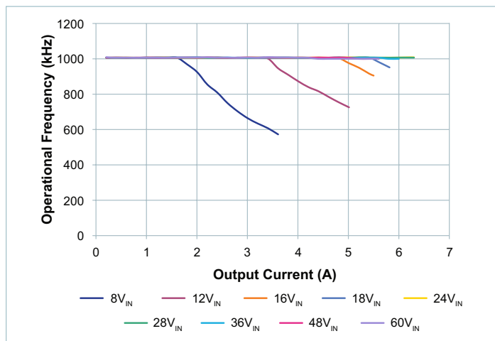
Figure 12 — Switching frequency vs. output current at 18V OUT
