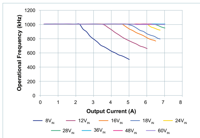
Figure 11 — Switching frequency vs. output current at 12V OUT
