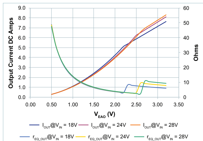
Figure 73 — r_{EQ\_OUT} vs. output current vs. V_{EAO} , V_{OUT} = 12V ; 18 – 28 V_{IN}
