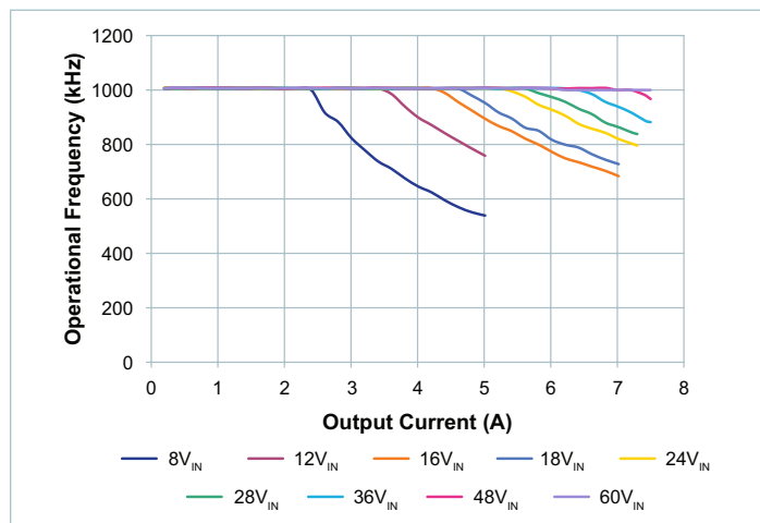
Figure 10 — Switching frequency vs. output current at 10V OUT
