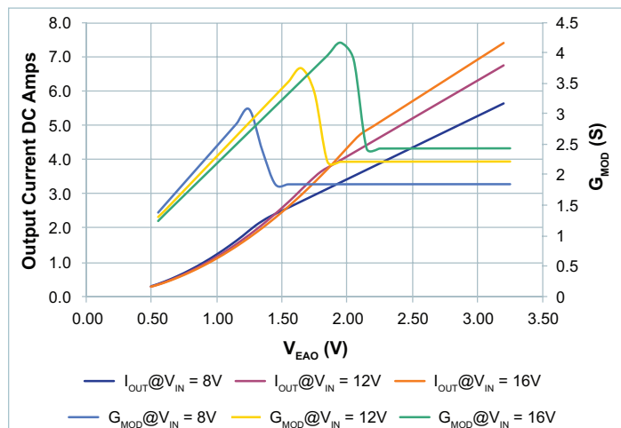
Figure 69 — G_{MOD} vs output current vs. V_{EAO} , V_{OUT} = 12V ; 8 – 16 V_{IN}
