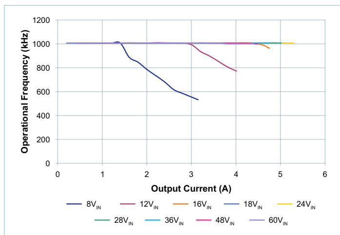
Figure 13 — Switching frequency vs. output current at 24V OUT
