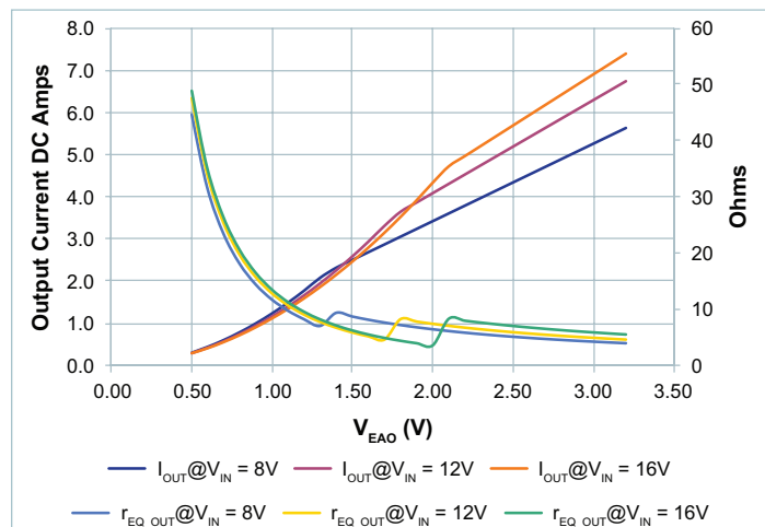
Figure 72 — r_{EQ\_OUT} vs. output current vs. V_{EAO} , V_{OUT} = 12V ; 8 – 16 V_{IN}
