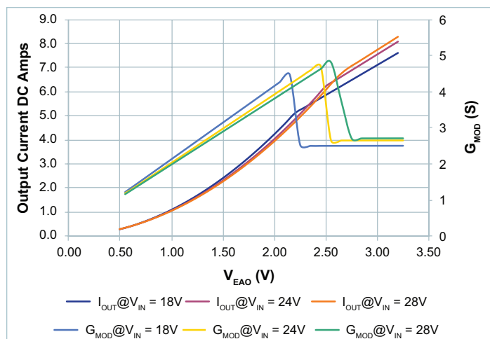
Figure 70 — G_{MOD} vs output current vs. V_{EAO} , V_{OUT} = 12V ; 18 – 28 V_{IN}
