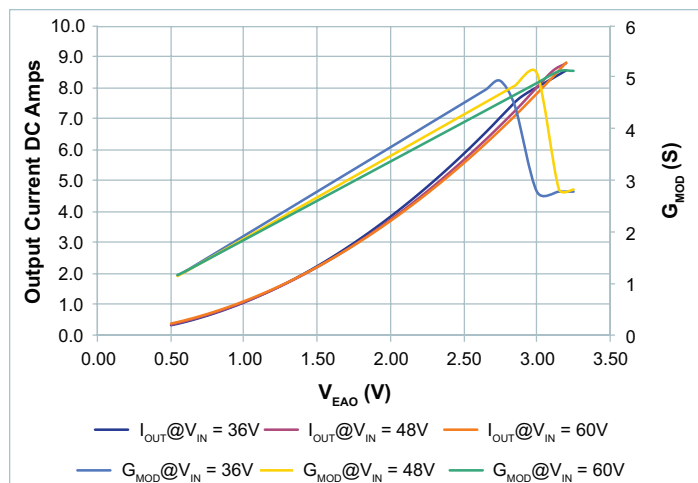
Figure 71 — G_{MOD} vs output current vs. V_{EAO} , V_{OUT} = 12V ; 36 – 60 V_{IN}
