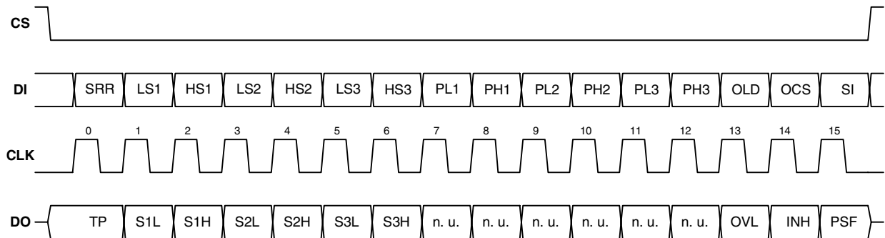
Figure 3. Data Transfer
