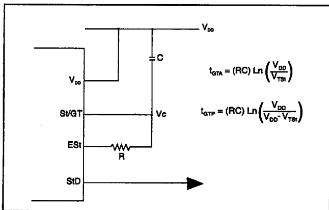
Figure 2 Basic Steering Circuit
