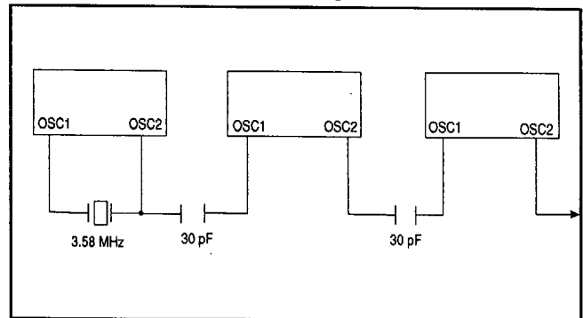
Figure 6 Common Crystal Connection
