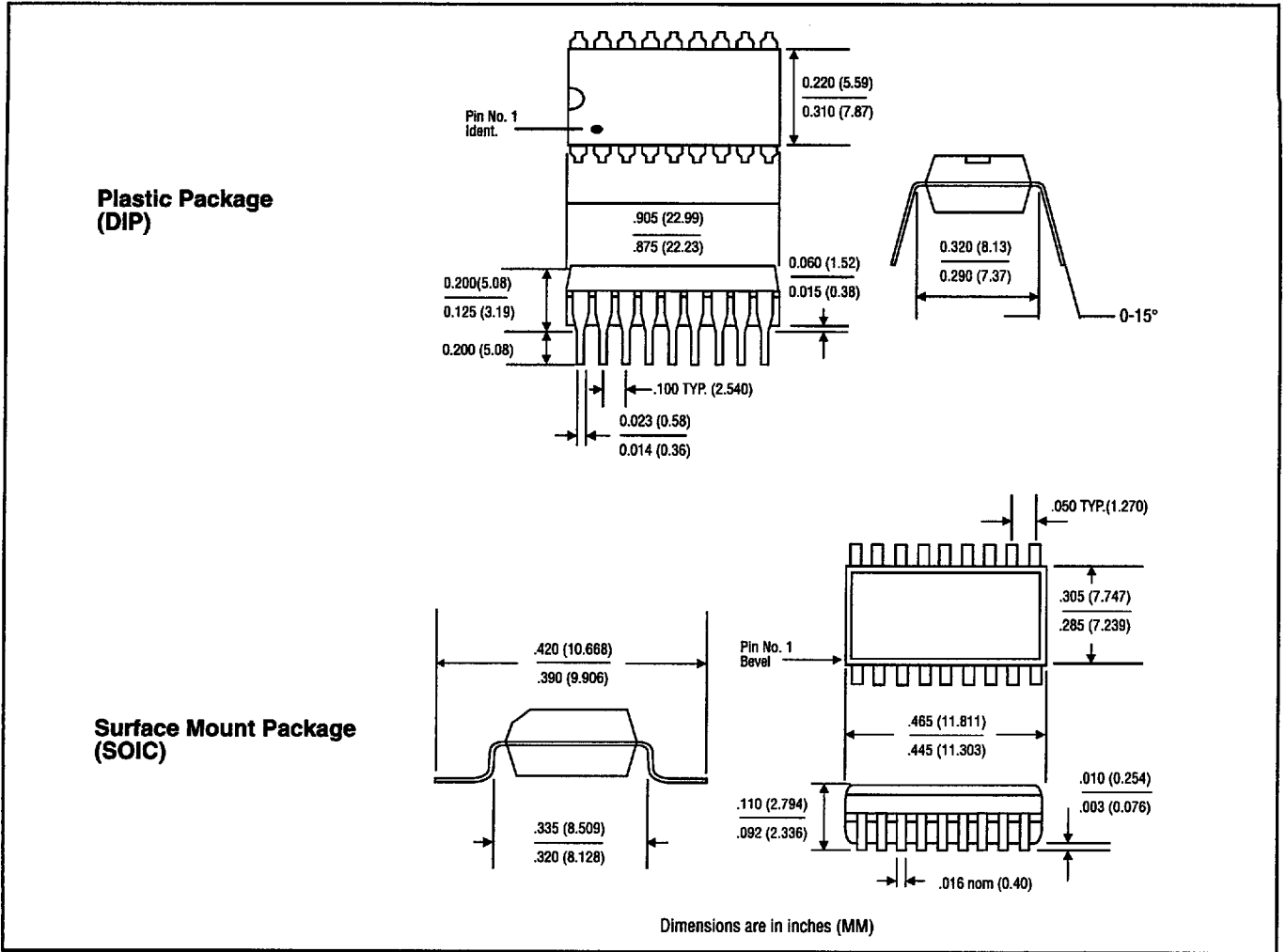
Figure 8 Package Dimensions
