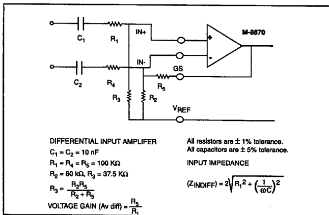
Figure 5 Differential Input Configuration
