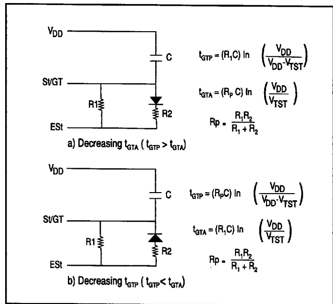
Figure 4 Guard Time Adjustment
