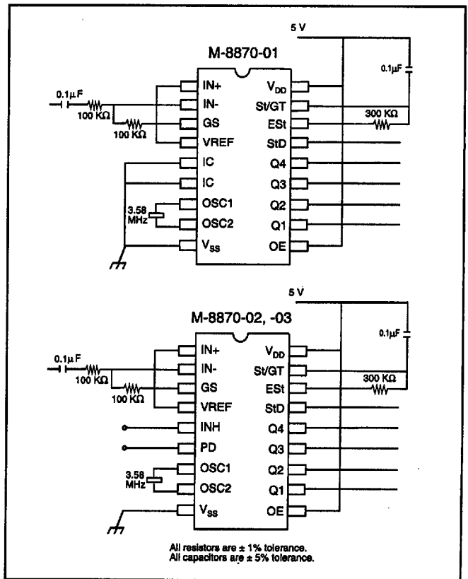
Figure 3 Single-Ended Input Configuration
