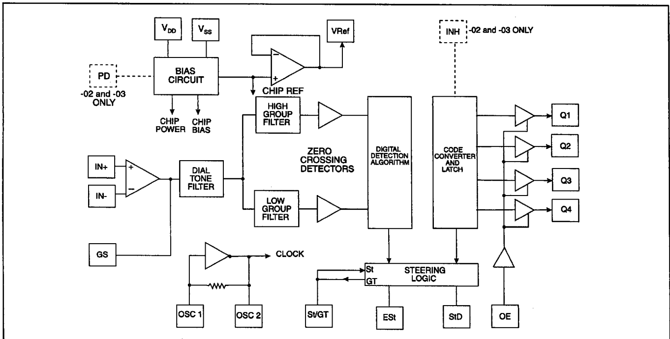
Figure 1 Block Diagram
