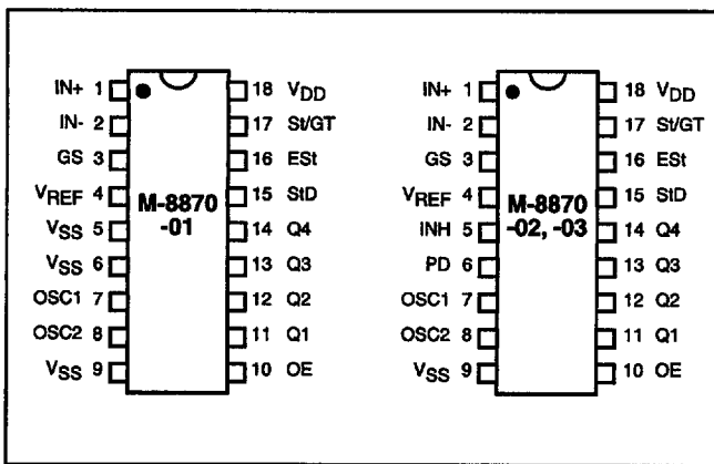
Figure 9 Pin Connections
