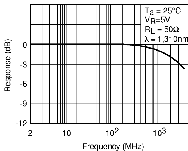
Fig. 6 Frequency Response
