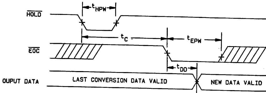
FIGURE 4. Conversion timing.
