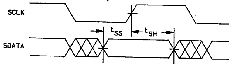
FIGURE 6. Serial output timing.
