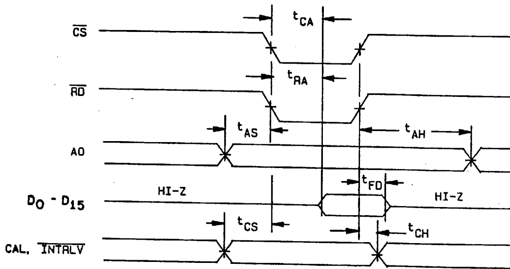
FIGURE 5. Read and calibration control timing.
