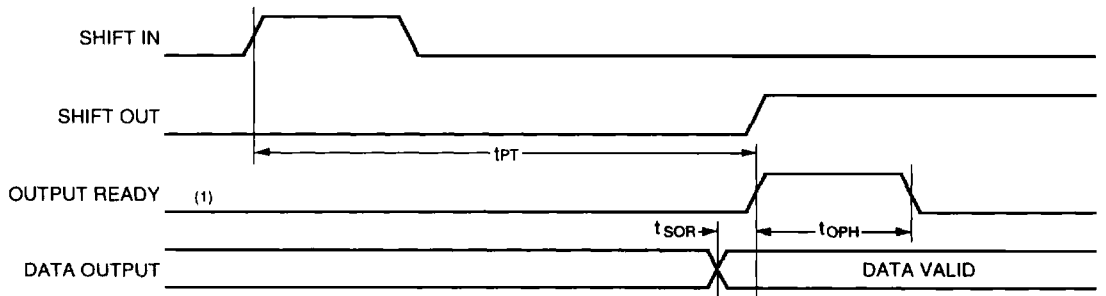
Figure 7. t_{PT} and t_{OPH} Specification
