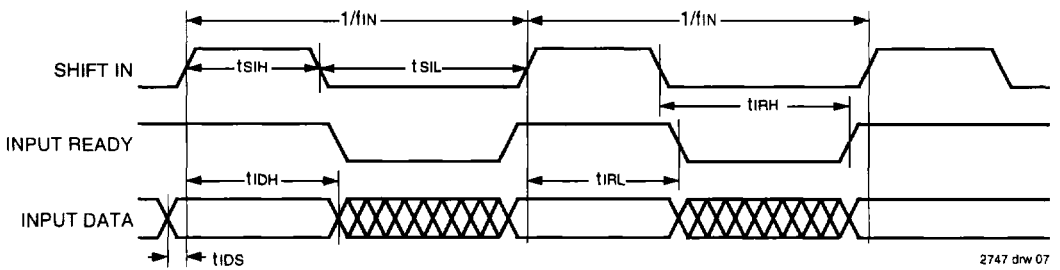
Figure 2. Input Timing
