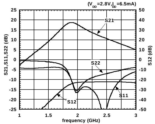
S21, S11, S22 vs. frequency
