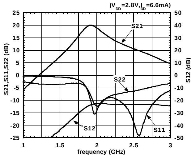
S21, S11, S22, S12 vs. frequency
