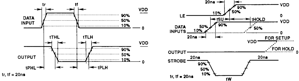
FIGURE 13. DYNAMIC WAVEFORMS
