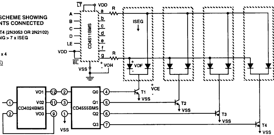
FIGURE 12. MULTIPLEXING WITH COMMON CATHODE 7-SEGMENT LED DISPLAYS (EXAMPLE HEWLETT-PACKARD 5082-7404 4 CHARACTER DISPLAY OR 4 DISCRETE MONOSANTO MAN 3 DISPLAYS)
