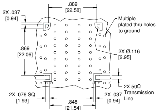
Dimensions are in Inches [Millimeters] XDL21-8-140 Mounting Footprint
