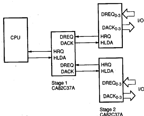
Figure 14 : CASCADED CA82C37As
