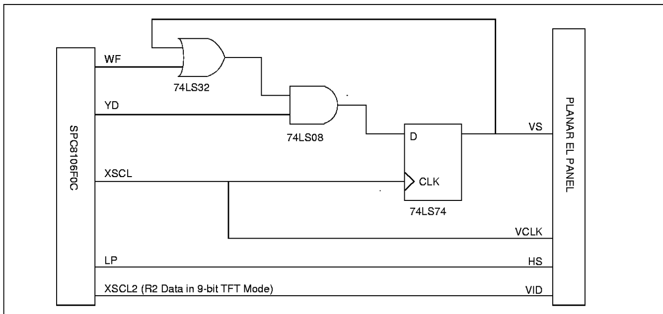
Figure 1: Planar EL Panel Connection to SPC8106F0C
