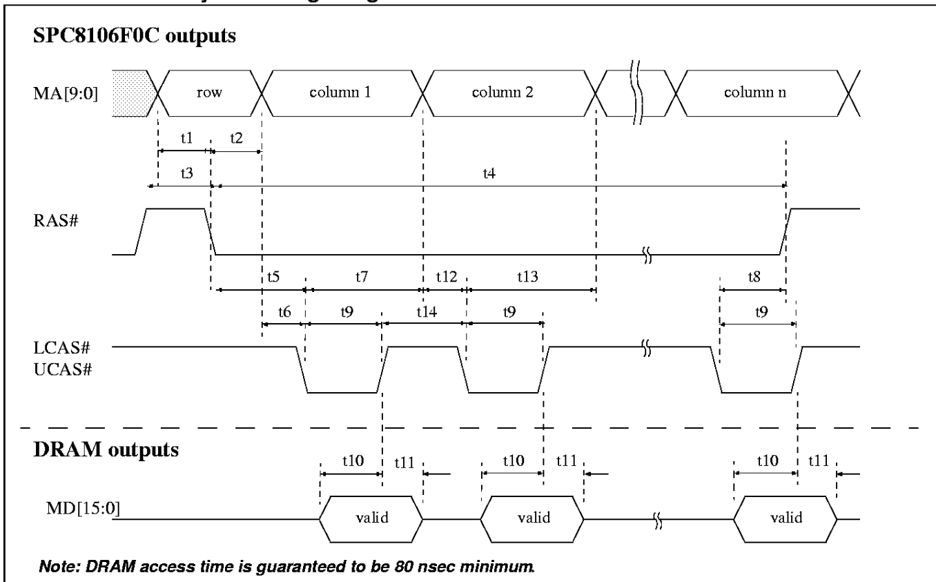
Figure 10: DRAM Read Cycle Timing - Page Mode
