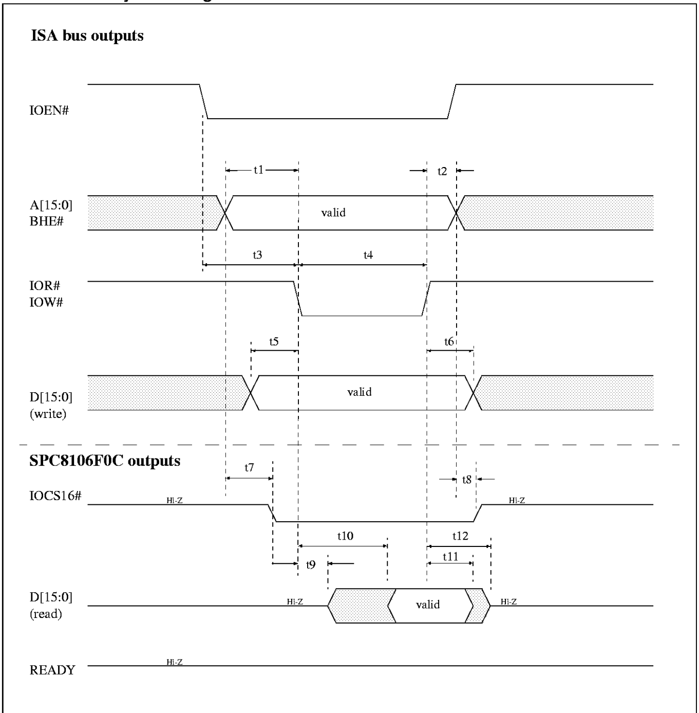
Figure 6: CPU Bus Cycle Timing - 16-Bit I/O
