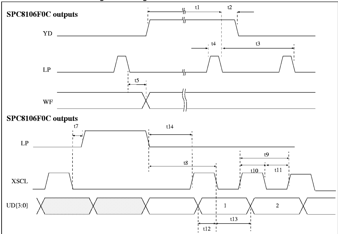
Figure 20: LCD Interface Timing - 4-Bit Single Monochrome Panel
