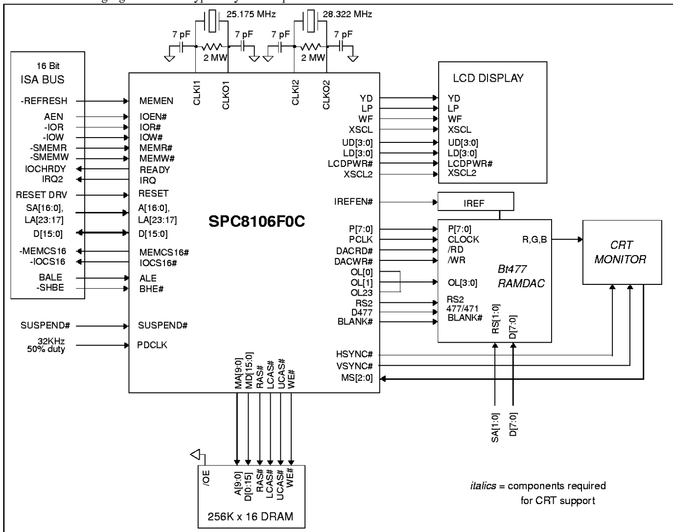
Figure 1: Typical System Implementation Diagram
