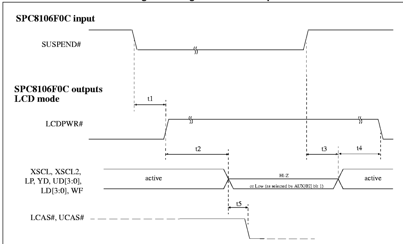
Figure 17: Suspend Mode LCD Signal Timing
