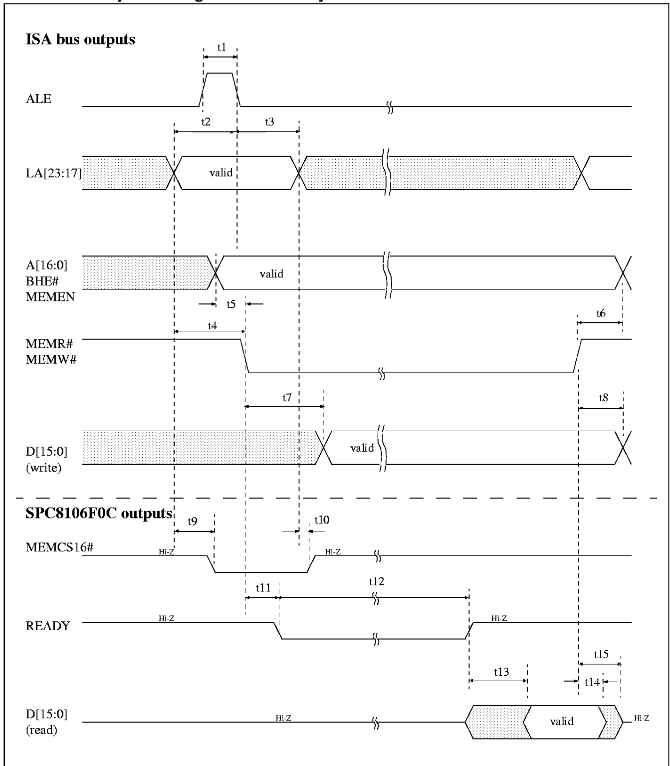
Figure 5: CPU Bus Cycle Timing - 16-Bit Memory
