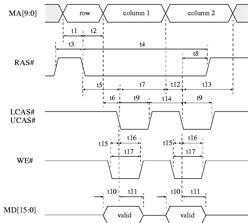
Figure 11: DRAM Write Cycle Timing
