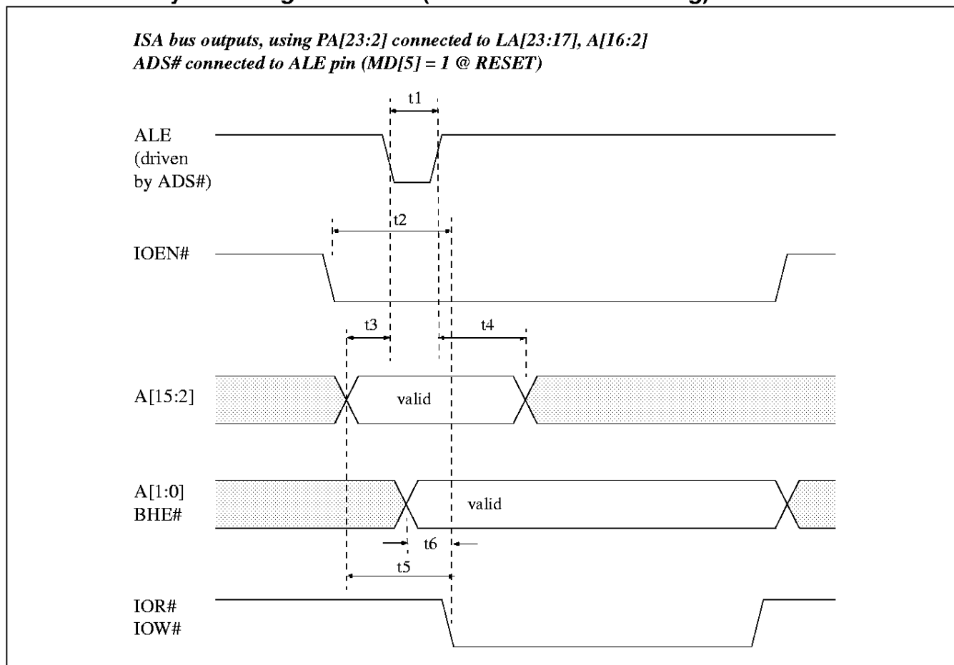
Figure 8: CPU Bus Cycle Timing - 16-Bit I/O - Modified Address Timing
