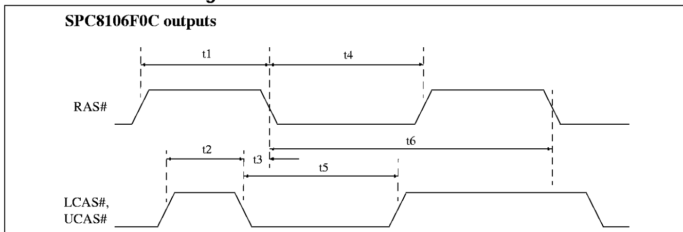
Figure 13: DRAM Refresh Timing II (Sequencer stopped)
