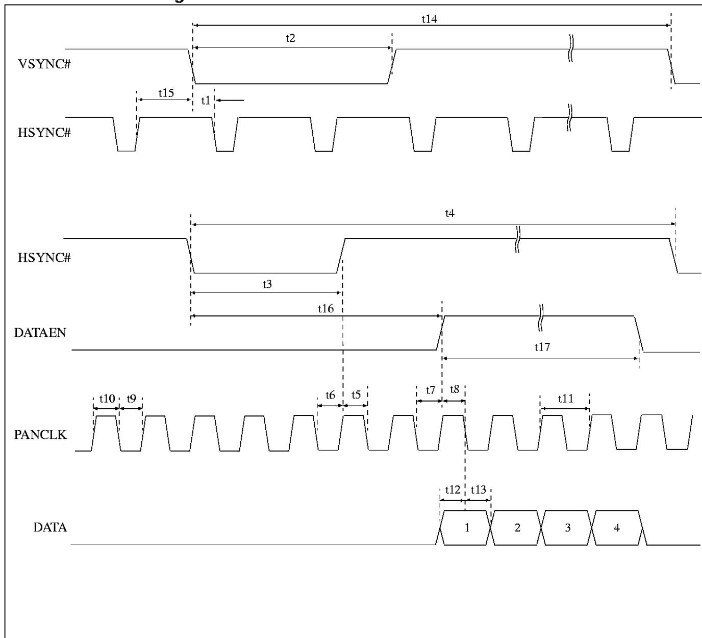
Figure 24: Interface Timing - TFT
