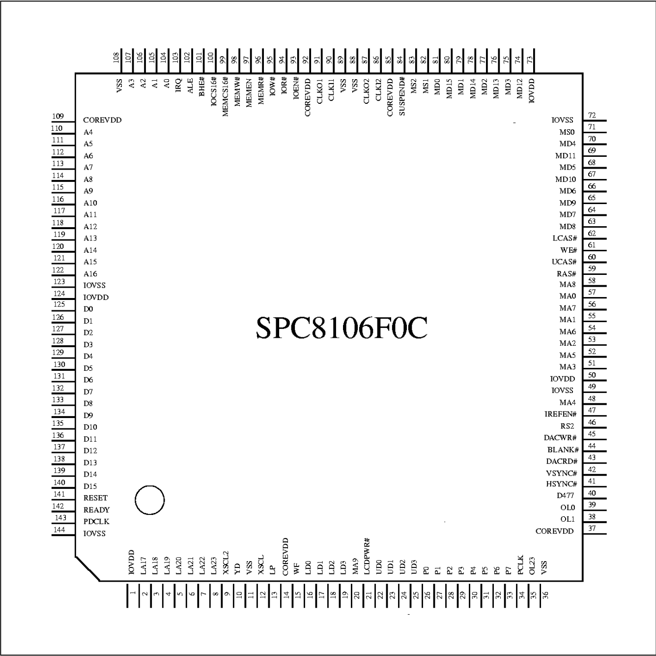
Figure 3: Pinout Diagram
