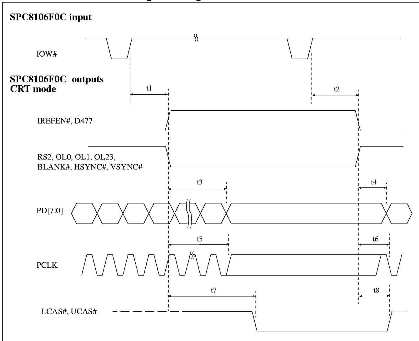
Figure 16: Power Save Mode CRT Signal Timing
