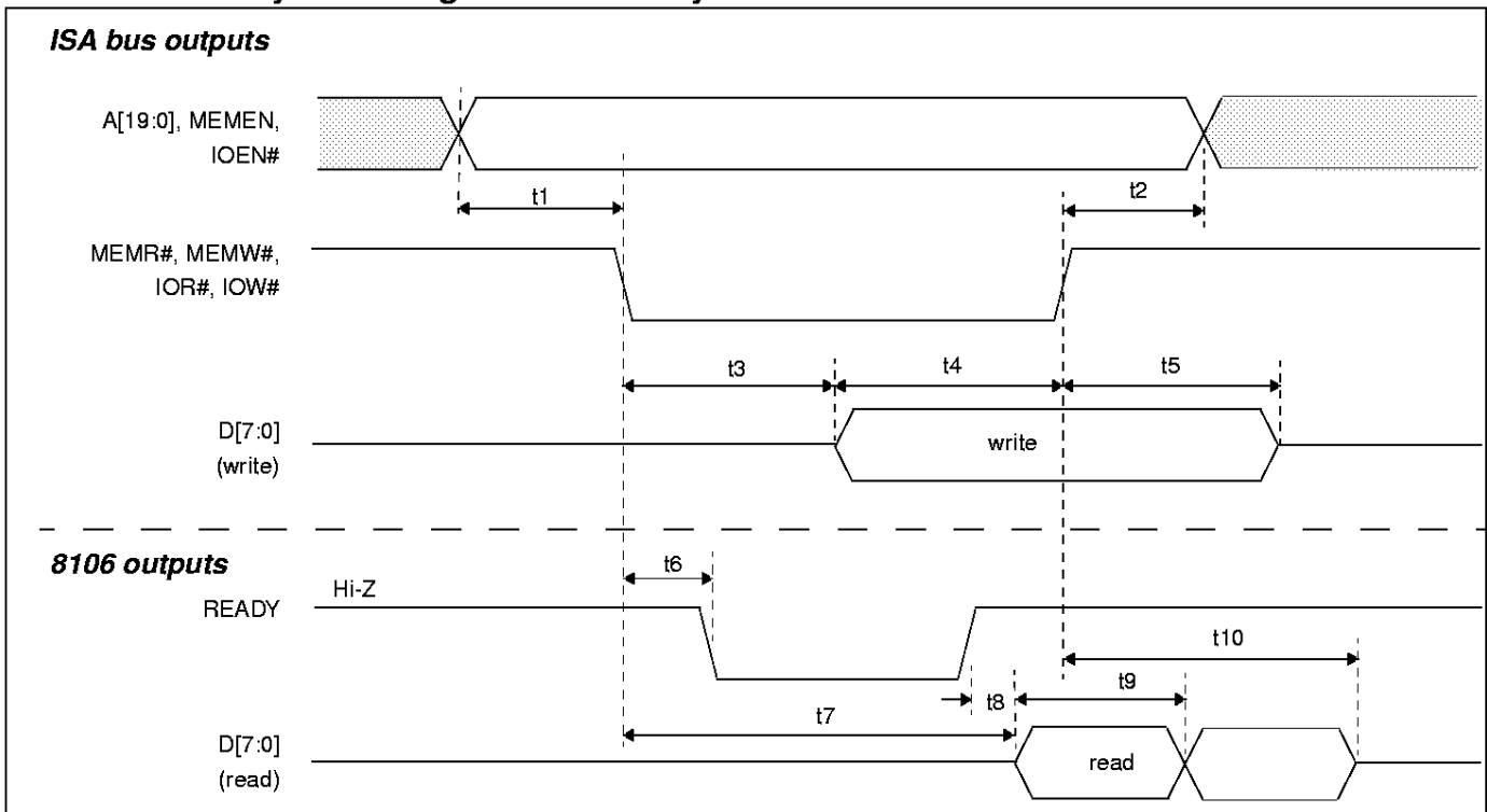
Figure 4: CPU Bus Cycle Timing - 8-Bit Memory
