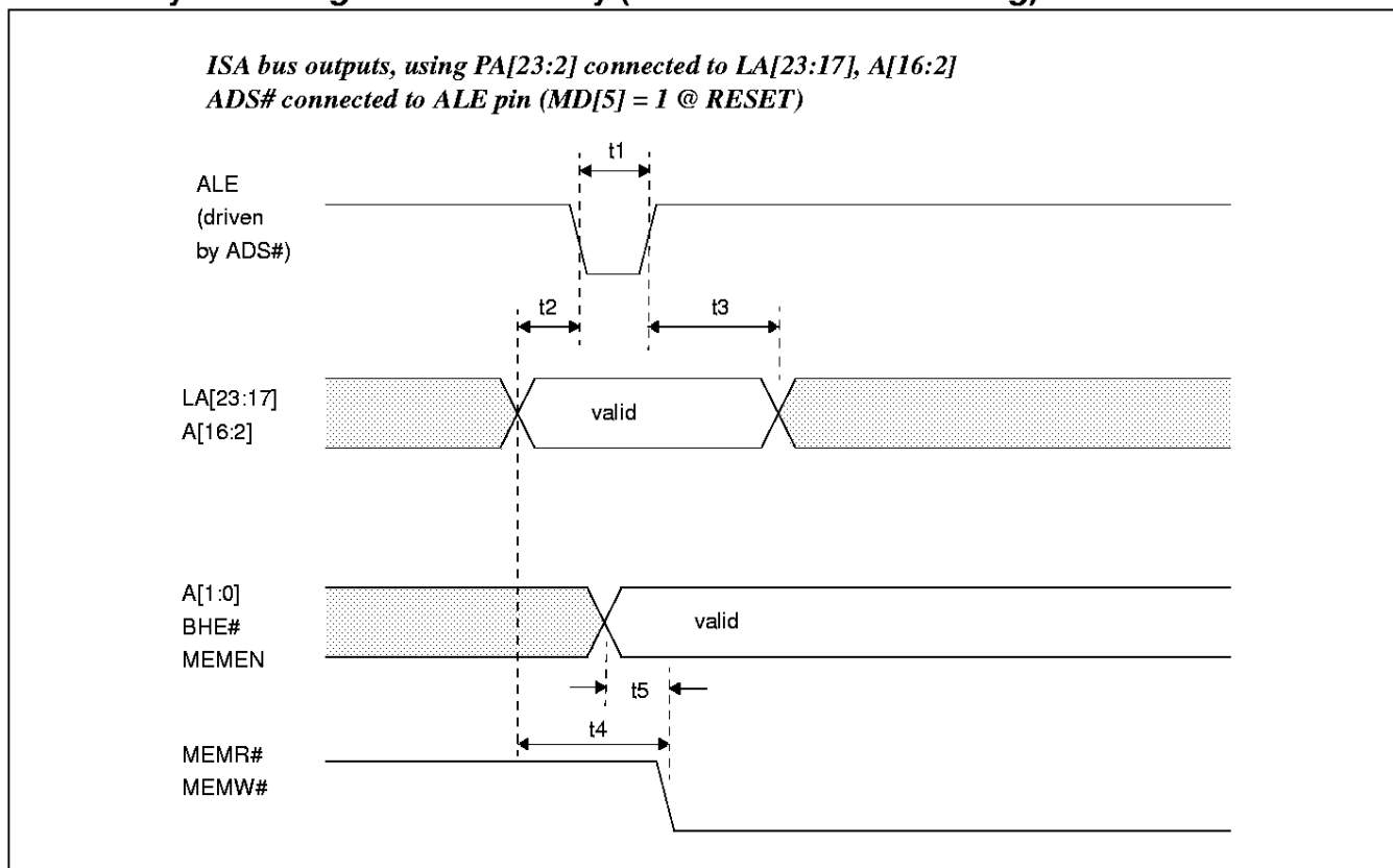
Figure 7: CPU Bus Cycle Timing - 16-Bit Memory, Modified Address Timing
