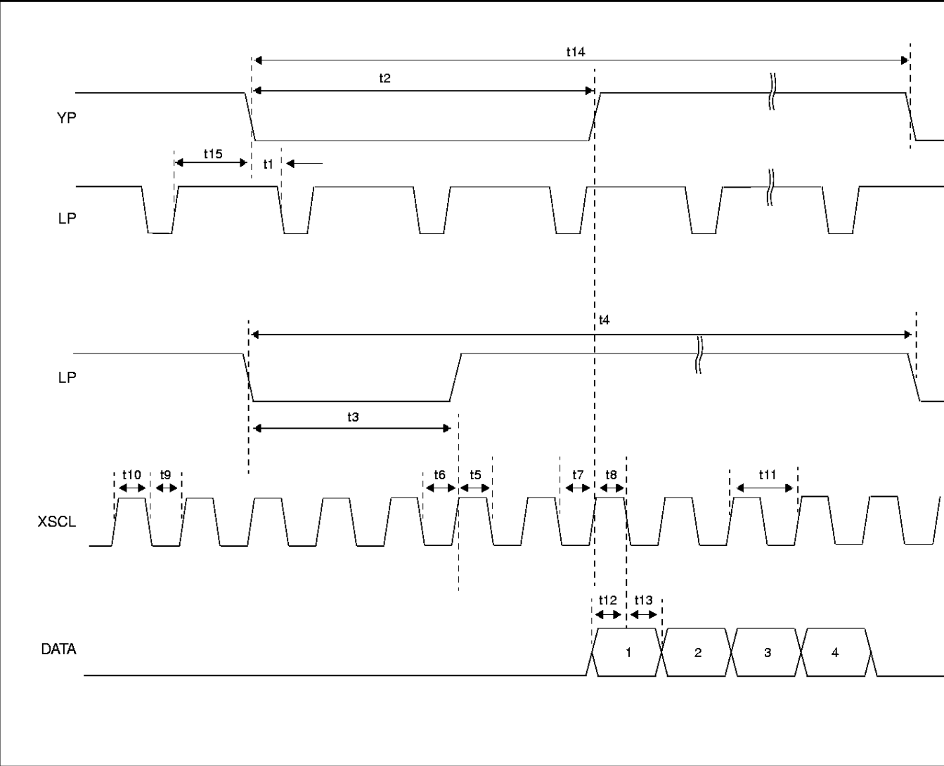
Figure 2: Interface Timing
