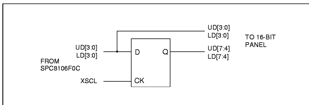
Figure 31: External Circuit Required for 16-Bit Panel When MD[7]=1 at RESET
