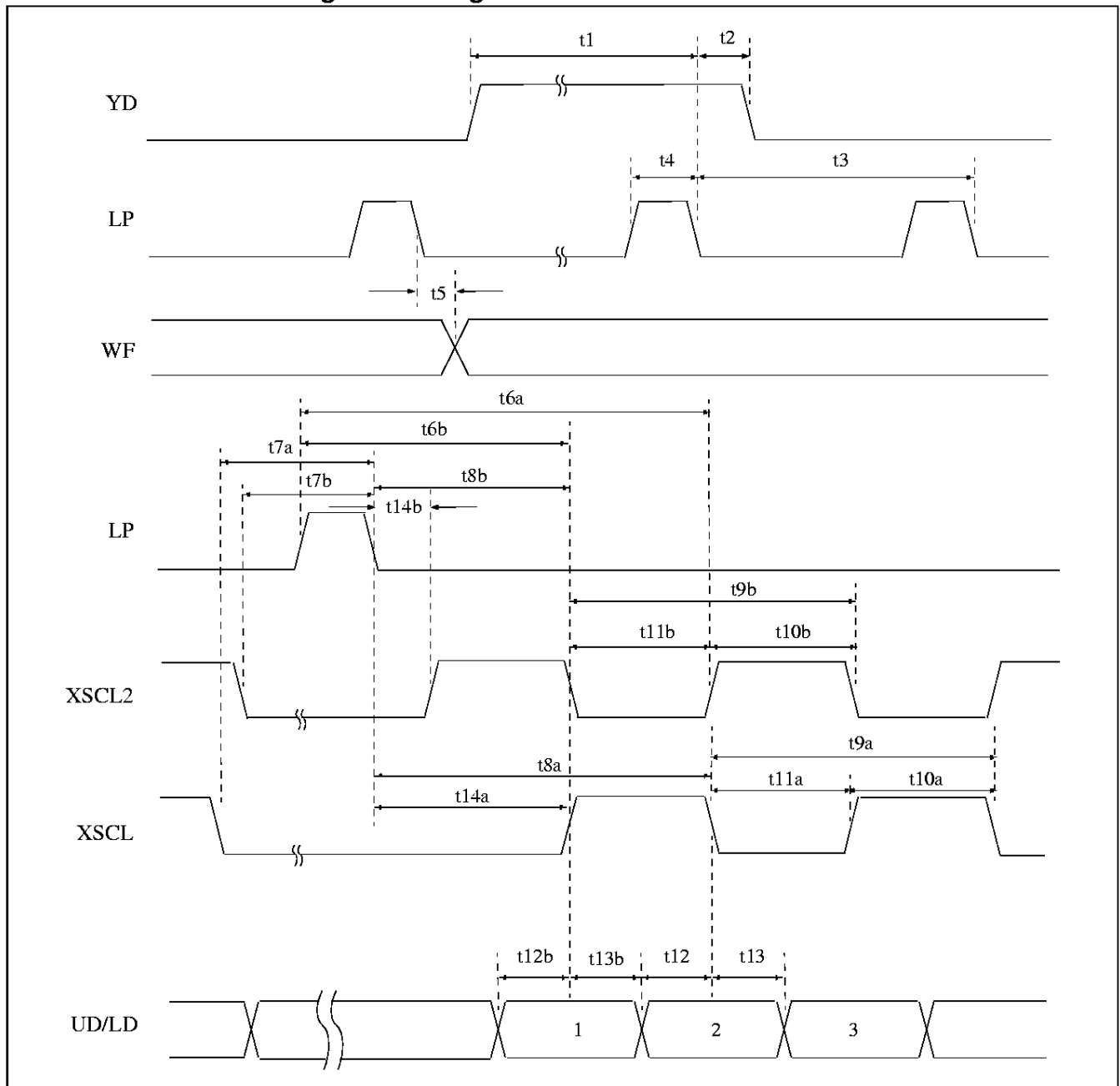
Figure 23: LCD Interface Timing - 8-Bit Single Color Panel
