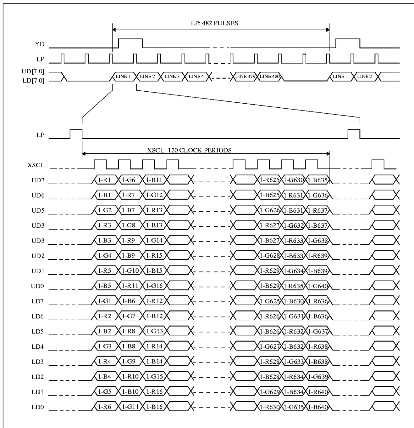
Figure 34: 16-Bit Single Color Panel Timing without External Circuit
