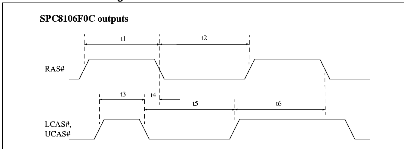
Figure 12: DRAM Refresh Timing I (Generated from CLKI, Sequencer running)
