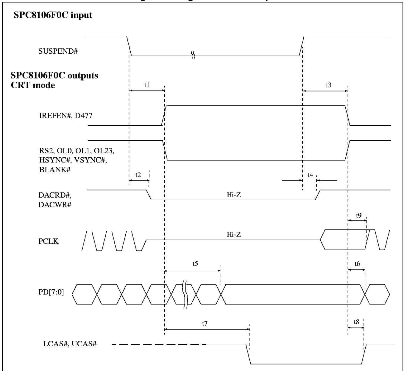
Figure 18: Suspend Mode CRT Signal Timing
