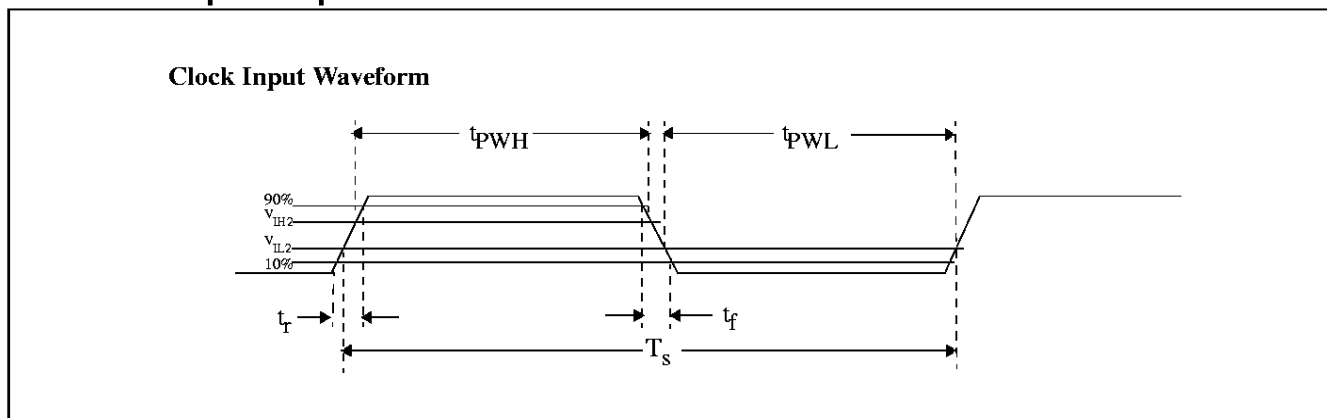
Figure 19: Clock Input Requirements
