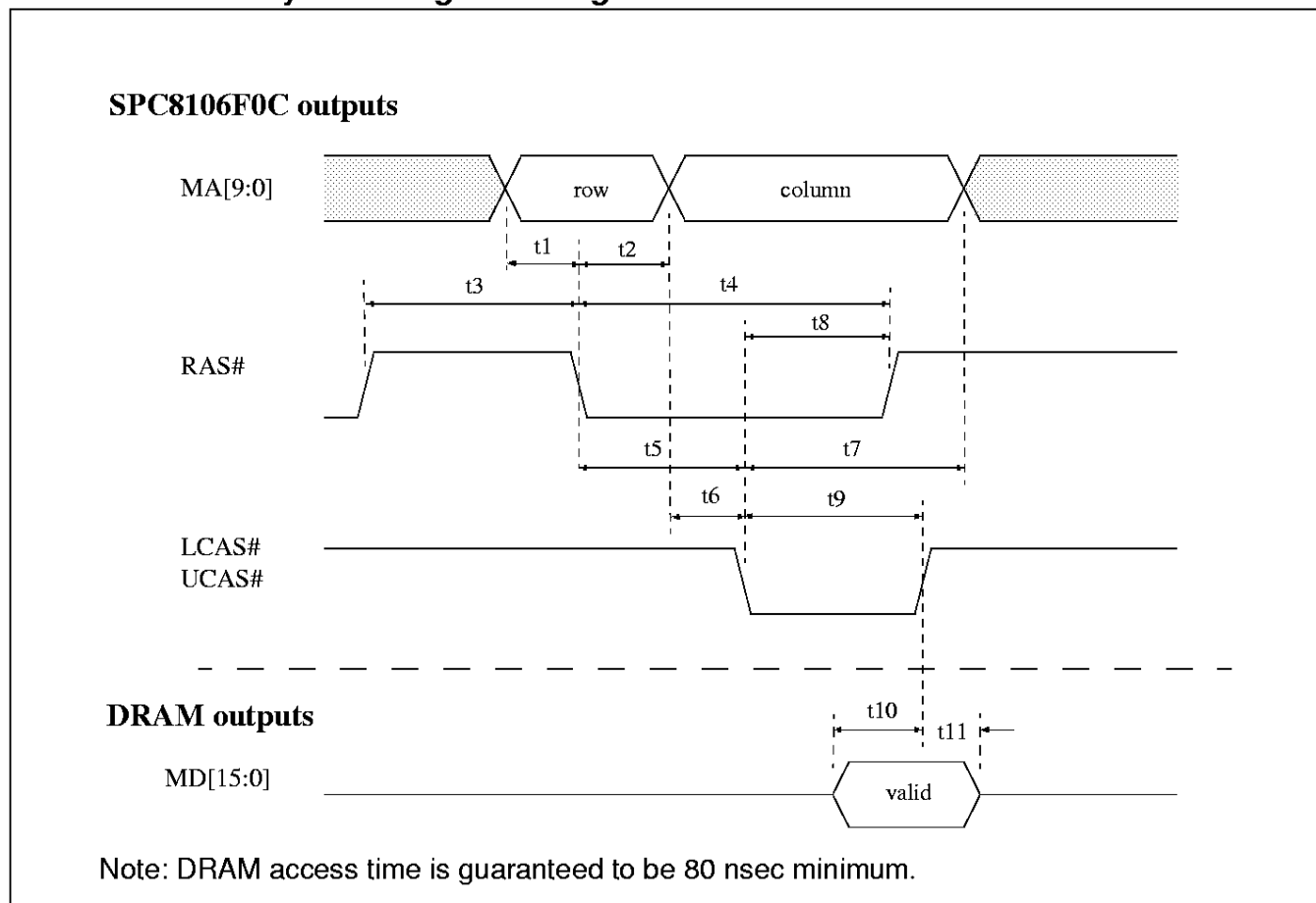
Figure 9: DRAM Read Cycle Timing - Non-Page Mode
