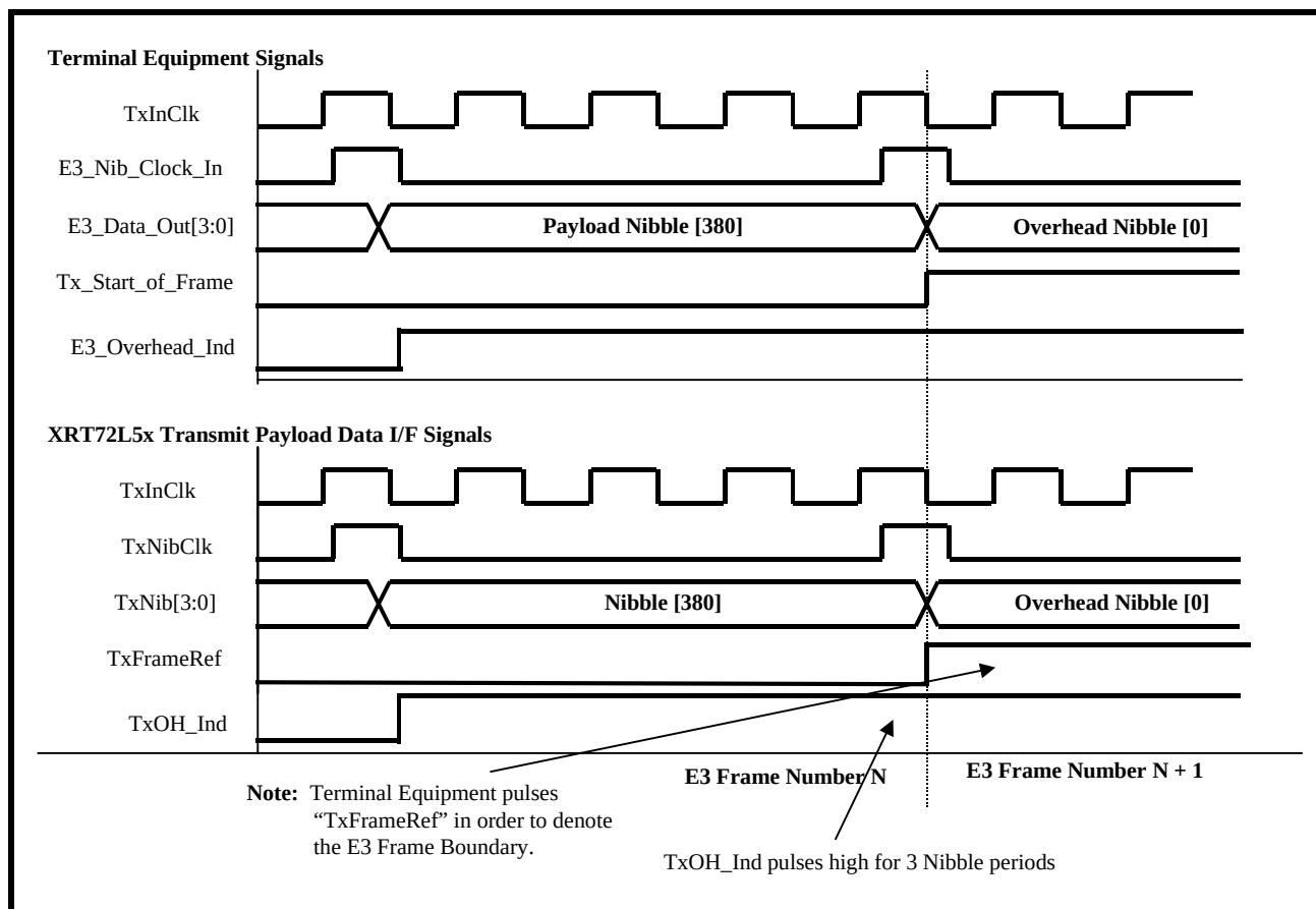
FIGURE 109. BEHAVIOR OF THE TERMINAL INTERFACE SIGNALS BETWEEN THE XRT72L56 AND THE TERMINAL EQUIPMENT (E3, MODE 5 OPERATION)
