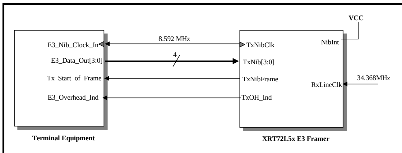
FIGURE 106. ILLUSTRATION OF THE TERMINAL EQUIPMENT BEING INTERFACED TO THE TRANSMIT PAYLOAD DATA INPUT INTERFACE BLOCK OF THE XRT72L56 FOR MODE 4 (NIBBLE-PARALLEL/LOOP-TIMED) OPERATION
