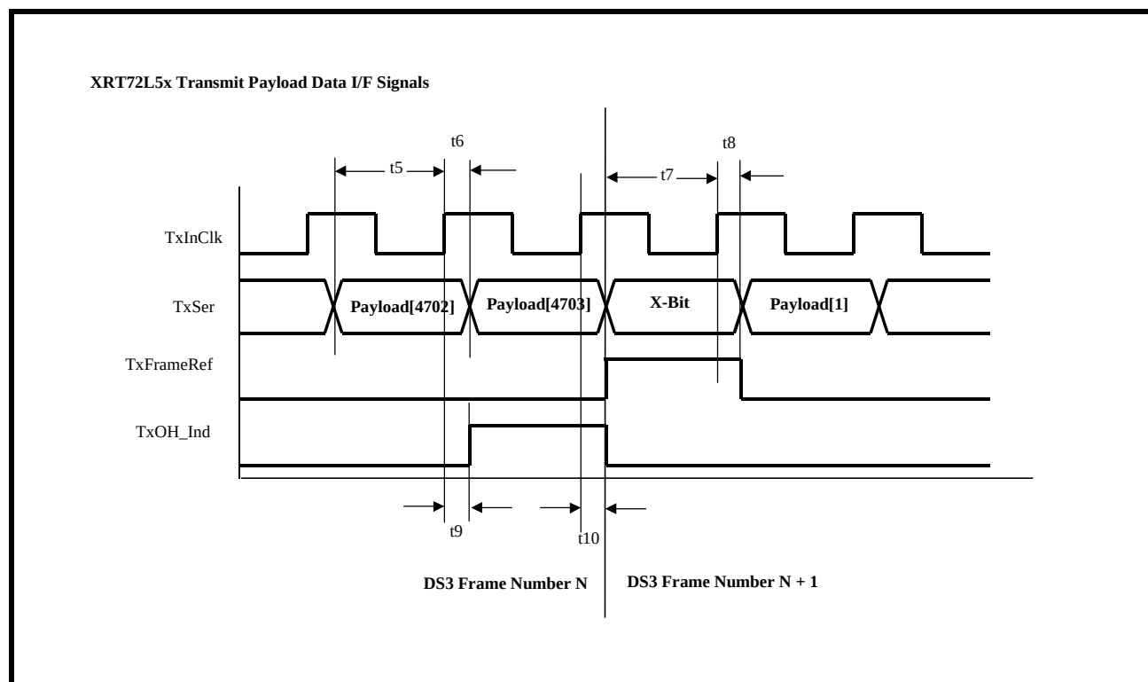
FIGURE 4. TIMING DIAGRAM FOR THE TRANSMIT PAYLOAD INPUT INTERFACE, WHEN THE XRT72L56 DEVICE IS OPERATING IN BOTH THE DS3 AND LOCAL-TIMING MODES
