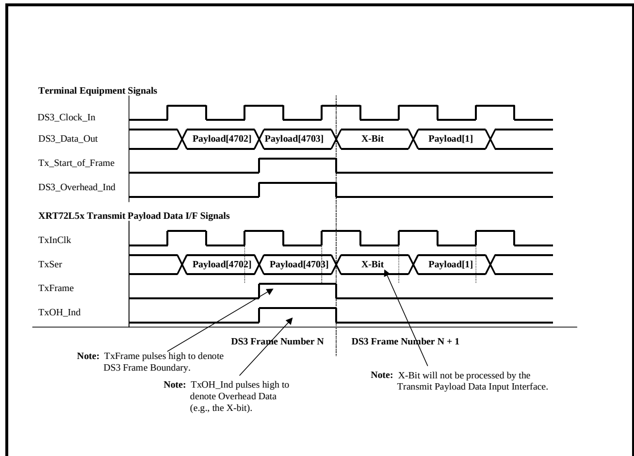
FIGURE 49. BEHAVIOR OF THE TERMINAL INTERFACE SIGNALS BETWEEN THE XRT72L56 AND THE TERMINAL EQUIPMENT (DS3 MODE 3 OPERATION)
