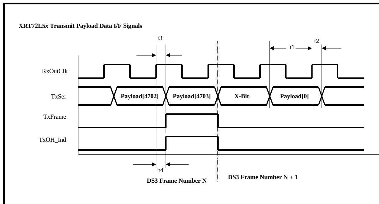
FIGURE 3. TIMING DIAGRAM FOR TRANSMIT PAYLOAD INPUT INTERFACE, WHEN THE XRT72L56 DEVICE IS OPERATING IN BOTH THE DS3 AND LOOP-TIMING MODES
