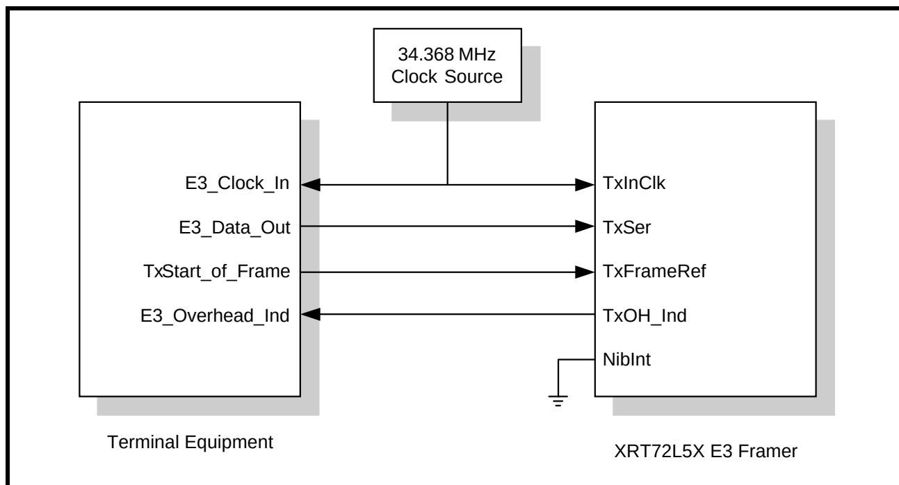
FIGURE 102. ILLUSTRATION OF THE TERMINAL EQUIPMENT BEING INTERFACED TO THE TRANSMIT PAYLOAD DATA INPUT INTERFACE BLOCK OF THE XRT72L56 FOR MODE 2 (SERIAL/LOCAL-TIMED/FRAME-SLAVE) OPERATION
