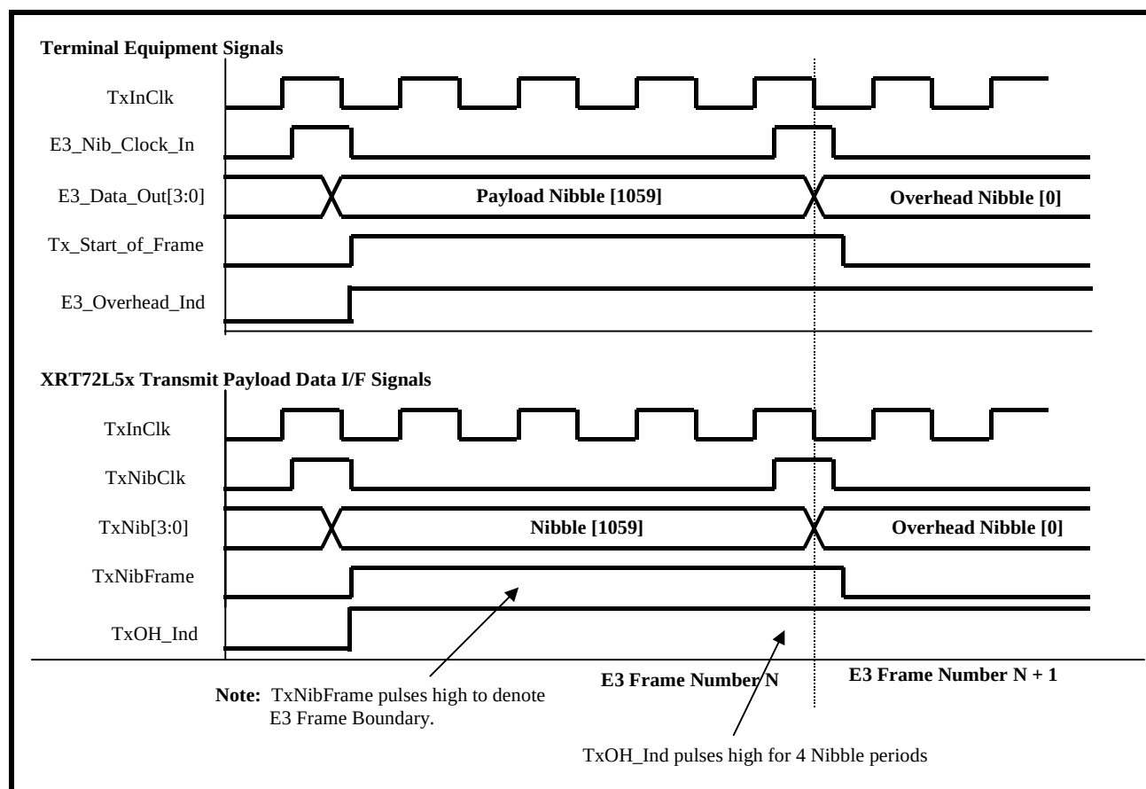
FIGURE 168. BEHAVIOR OF THE TERMINAL INTERFACE SIGNALS BETWEEN THE XRT72L56 AND THE TERMINAL EQUIPMENT (E3 MODE 6 OPERATION)
