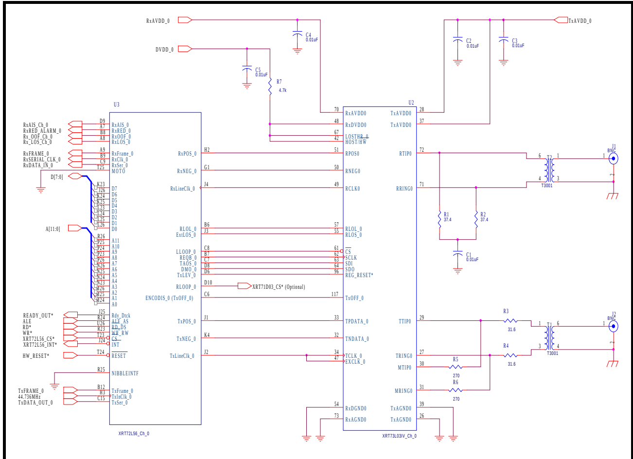
FIGURE 39. SCHEMATIC DEPICTING HOW TO INTERFACE THE XRT72L56 DS3/E3 FRAMER IC TO THE XRT73L03 DS3/E3/STS-1 LIU IC (ONE CHANNEL SHOWN)
