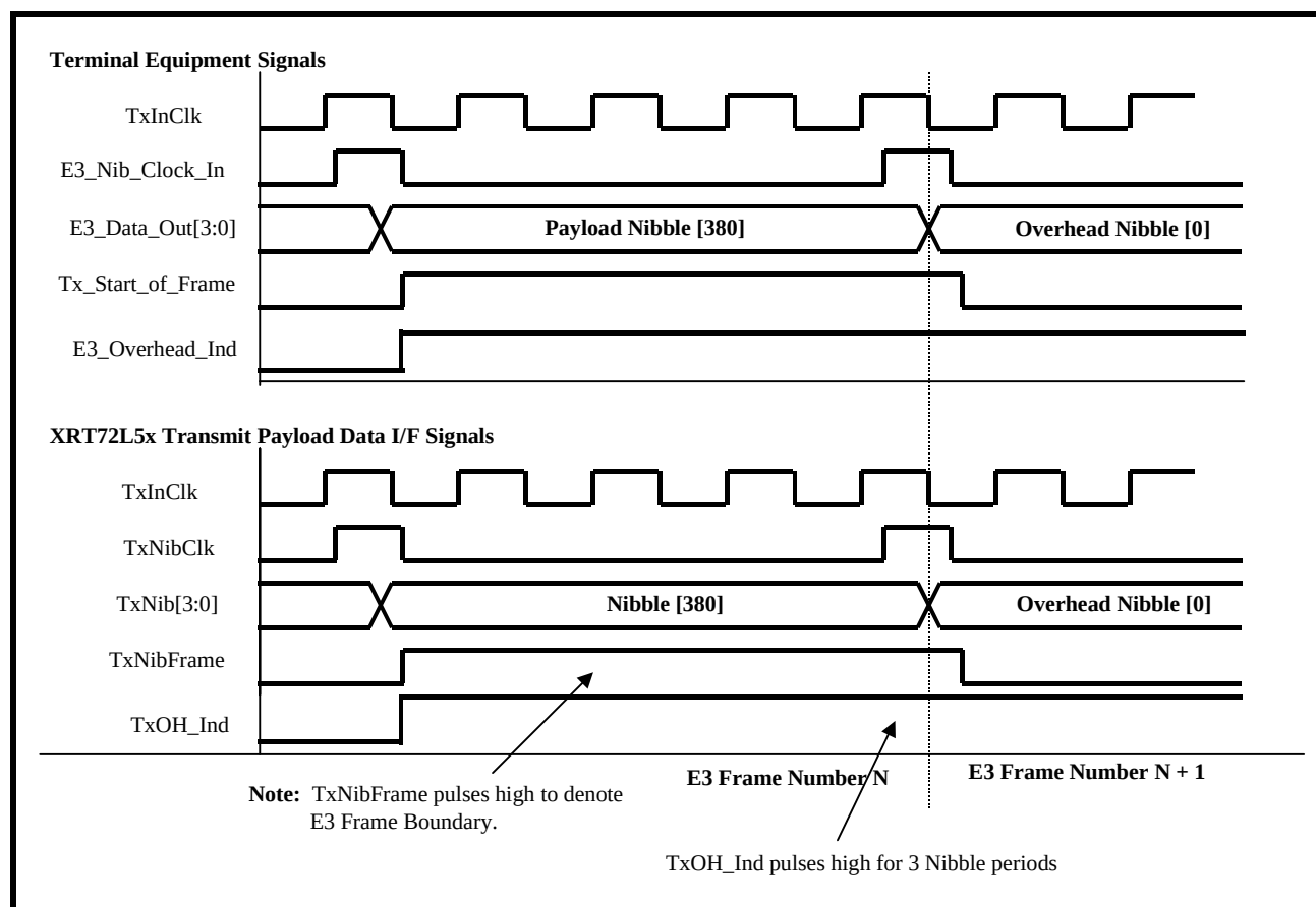
FIGURE 111. BEHAVIOR OF THE TERMINAL INTERFACE SIGNALS BETWEEN THE XRT72L56 AND THE TERMINAL EQUIPMENT (E3 MODE 6 OPERATION)
