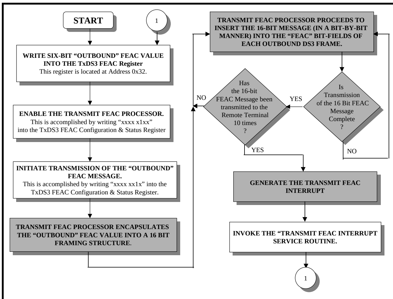
FIGURE 61. A FLOW CHART DEPICTING HOW TO TRANSMIT A FEAC MESSAGE VIA THE FEAC TRANSMITTER
