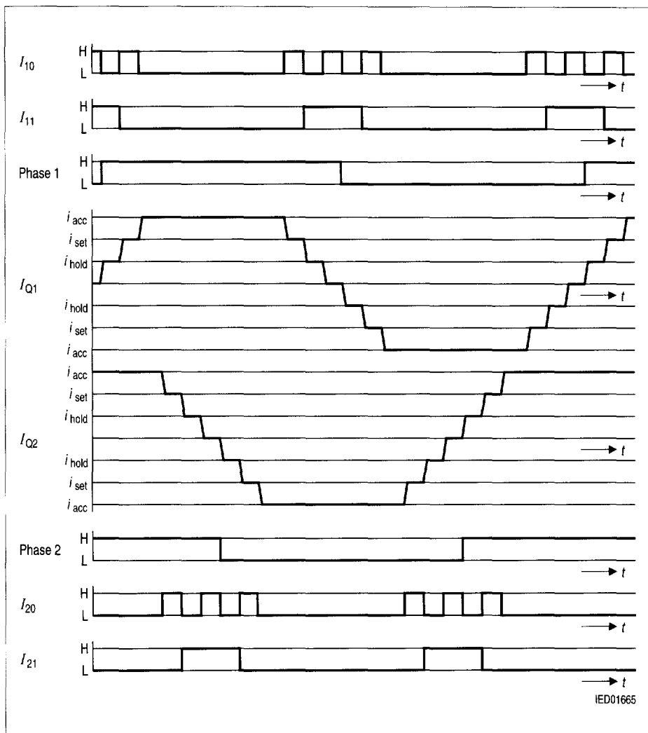
Figure 9 Mini-Step Operation
