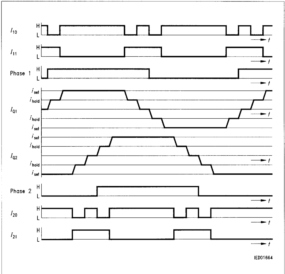
Figure 8 Quarter-Step Operation
