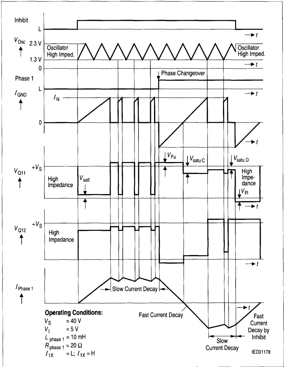
Figure 11 Phase Reversal and Inhibit
