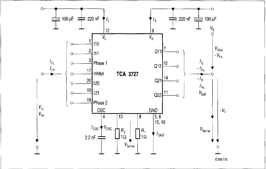
Figure 4 Test Circuit
