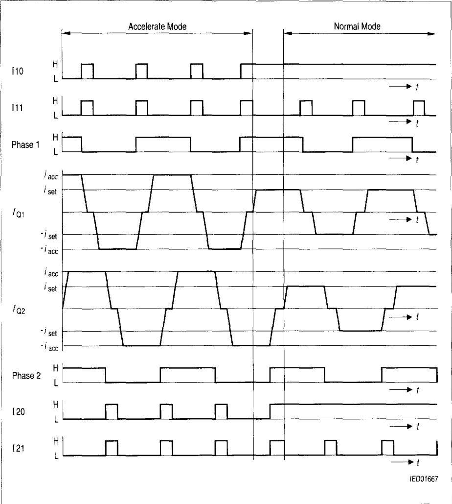
Figure 7 Half-Step Operation
