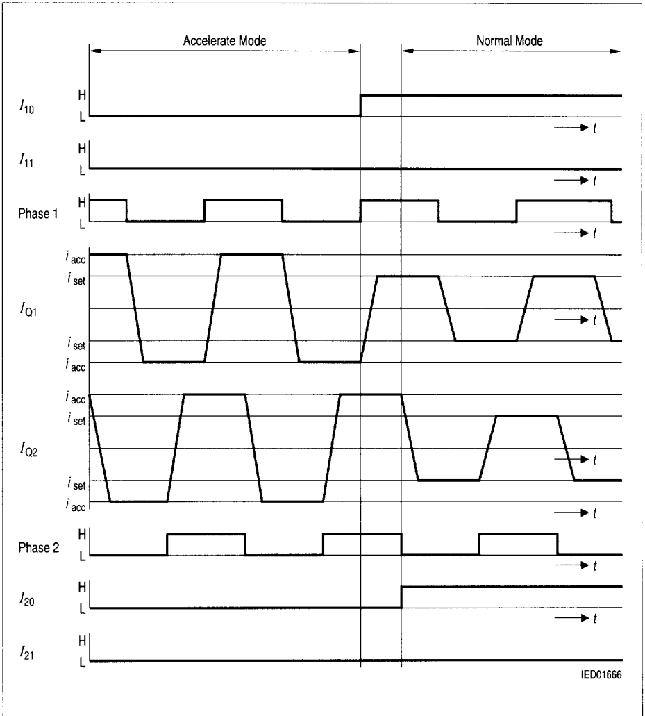
Figure 6 Full-Step Operation
