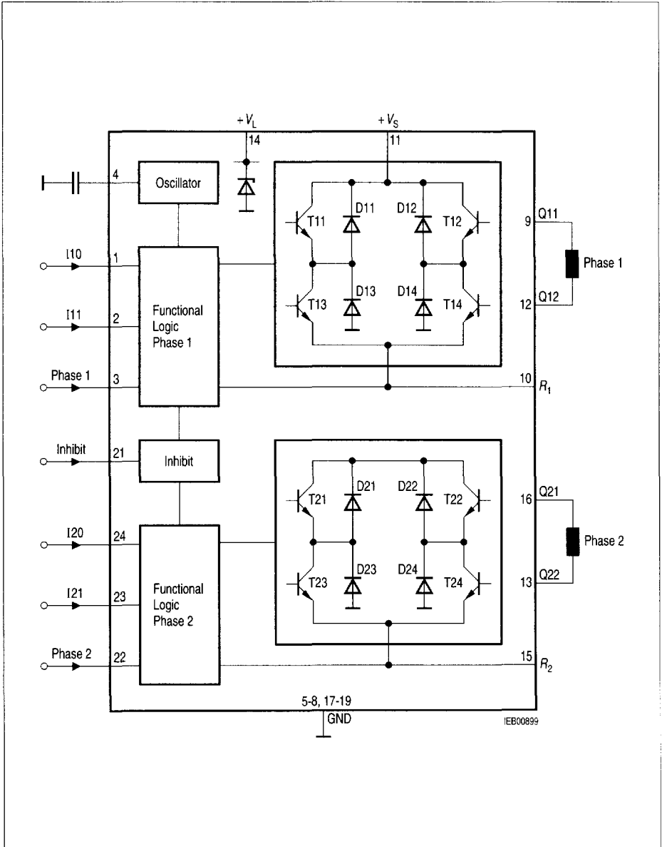
Figure 3 Block Diagram TCA 3727 G
