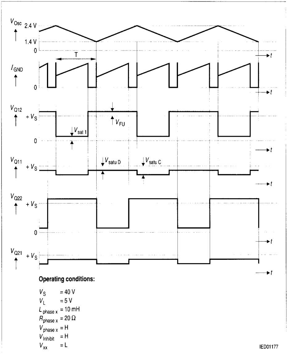
Figure 10 Current Control
