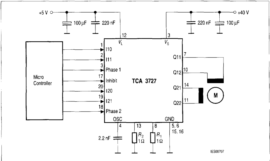
Figure 5 Application Circuit
