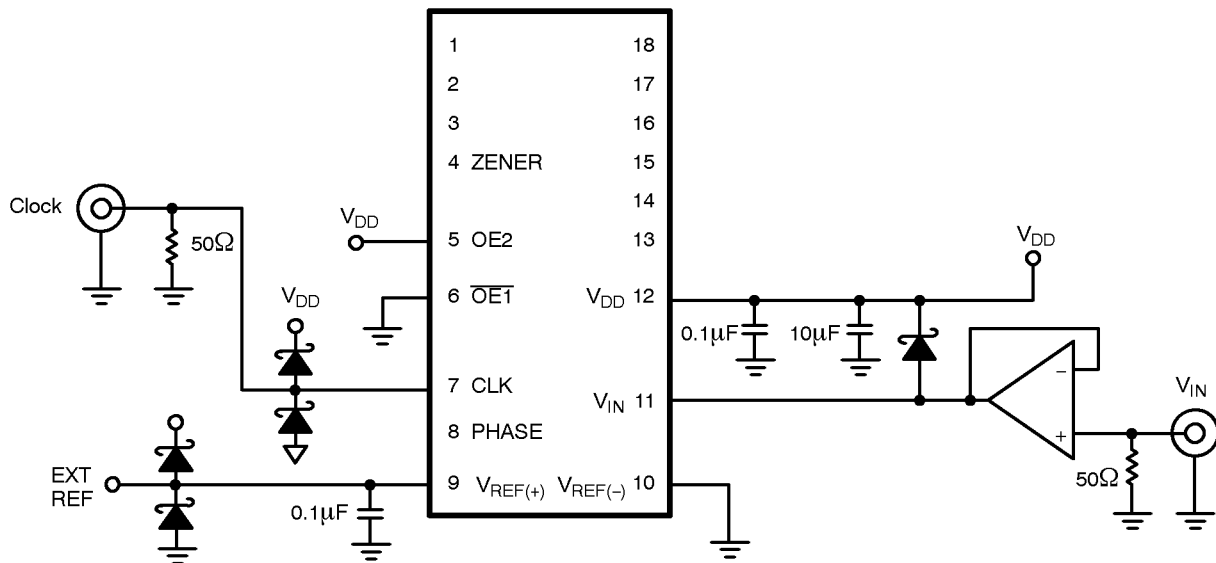
Figure 7. Typical Connections
