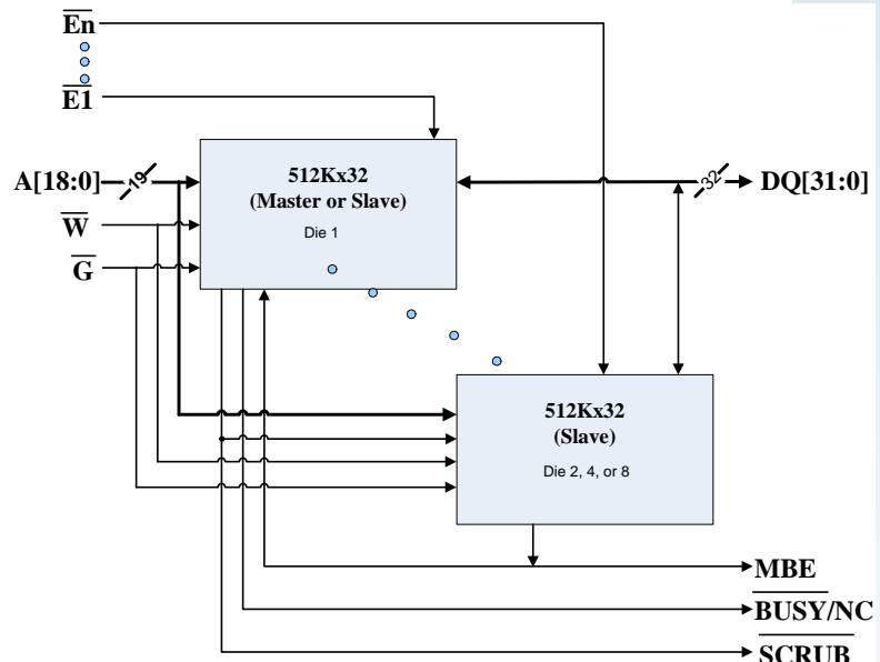
Figure 1. Block Diagram
