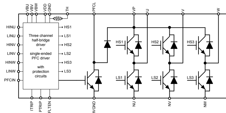
Figure 1. Functional Diagram
