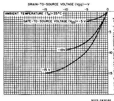
Fig. 6 - Minimum carry or borrow output high (source) current characteristics.
