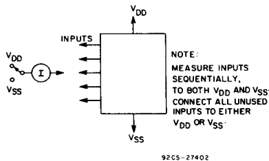
Fig. 13 - Input current.
