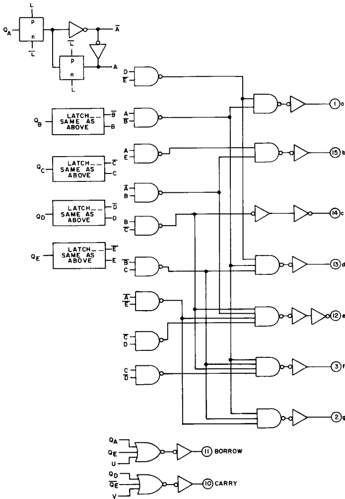
Fig. 2 - Logic diagram with flip-flop and output-driver details.
