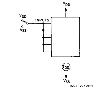
Fig. 12 - Quiescent device current.
