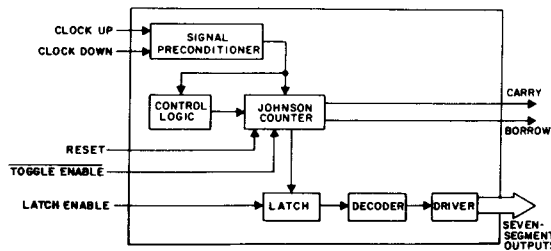
Fig. 1 - Functional diagram.
