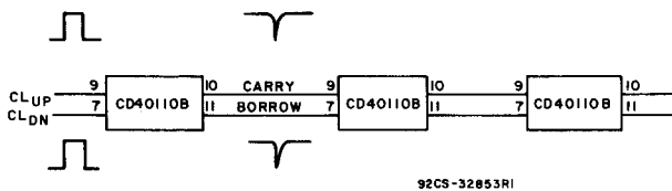
Fig. 15 - Cascading diagram.
