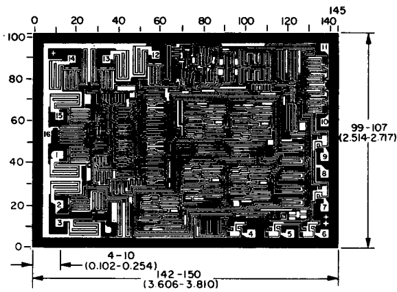
Dimensions and pad layout for CD40110B.
