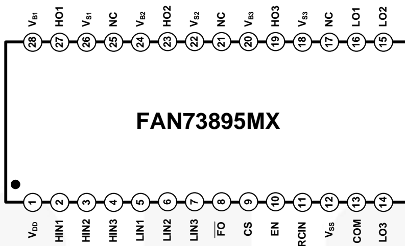
Figure 4. Pin Assignments
