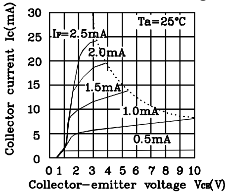
Fig.2 Collector Current vs. Collector-emitter Voltage
