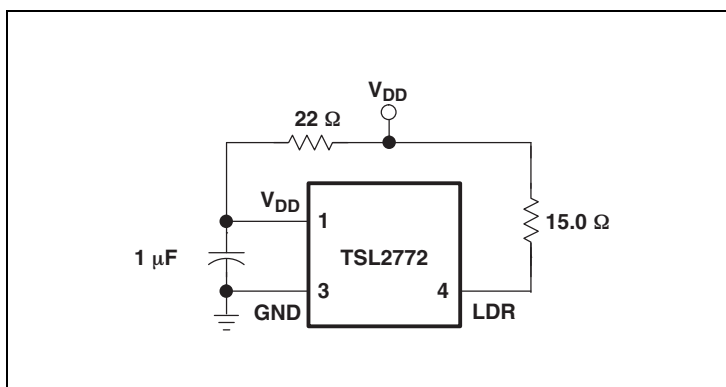
Figure 10: Proximity Noise Test Circuit
