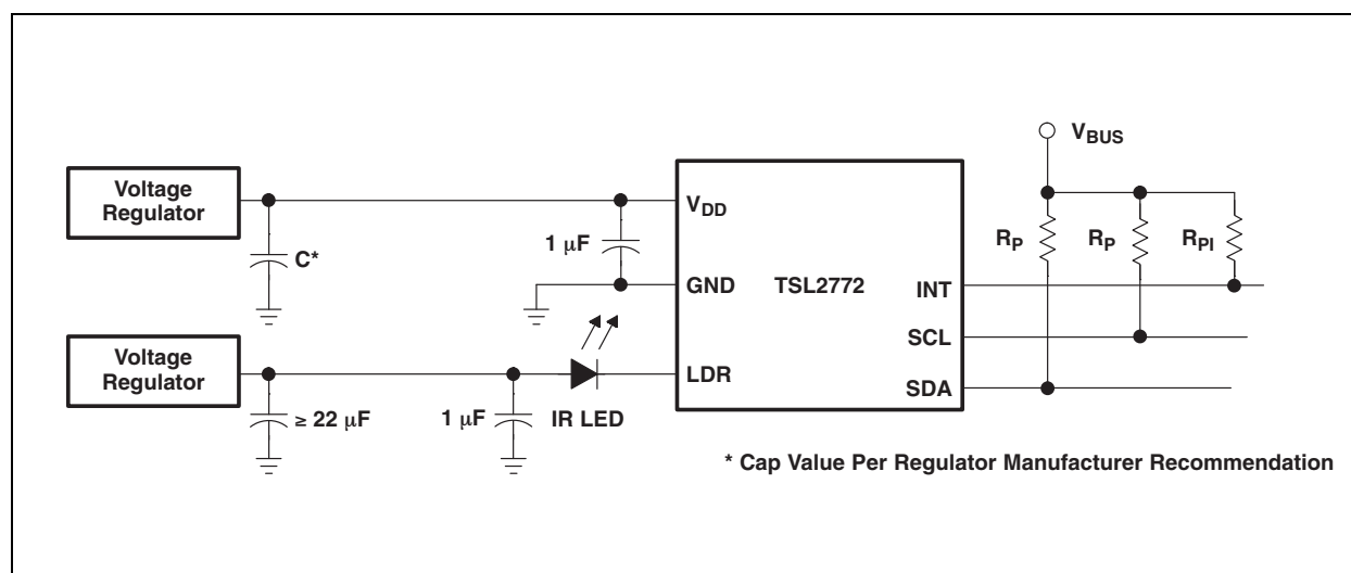
Figure 47: Proximity Sensing Using Separate Power Supplies
