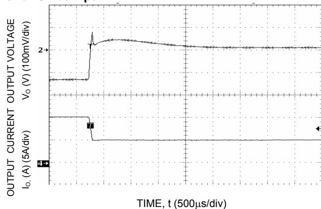
Figure 6. Typical Transient Response to Step decrease in Output Load from 10A to 5A at Room Temperature and 48 Vdc Input.
