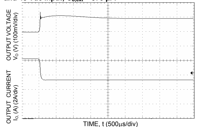
Figure 14. Typical Transient Response to Step decrease in Output Load from 8.1A to 5.3A at Room Temperature and 48 Vdc Input; C_{o,ext} = 370 \mu F .
