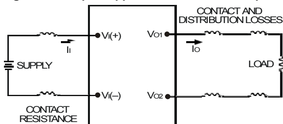
Figure 18. Output Ripple and Noise Test Setup.
