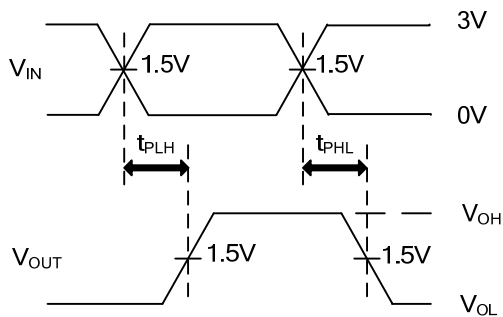
PROPAGATION DELAY TIMES
