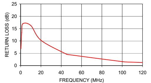
T16-1 INPUT RETURN LOSS
