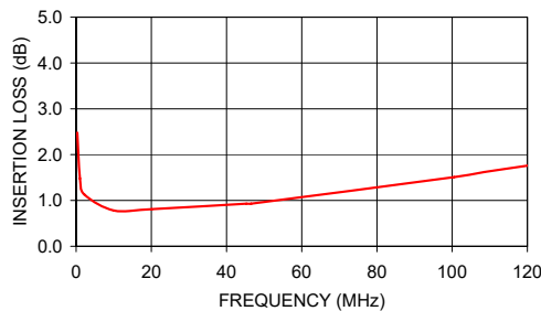
T16-1 INSERTION LOSS
