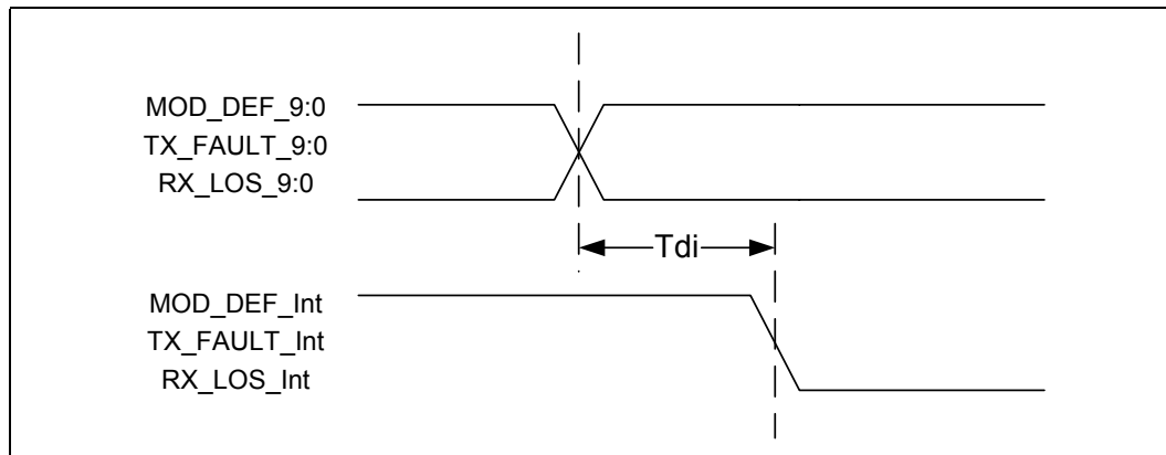
Figure 33. GBIC Interrupt Timing
