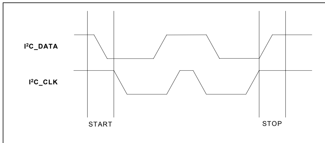
Figure 17. Start and Stop Definition Timing Diagram
