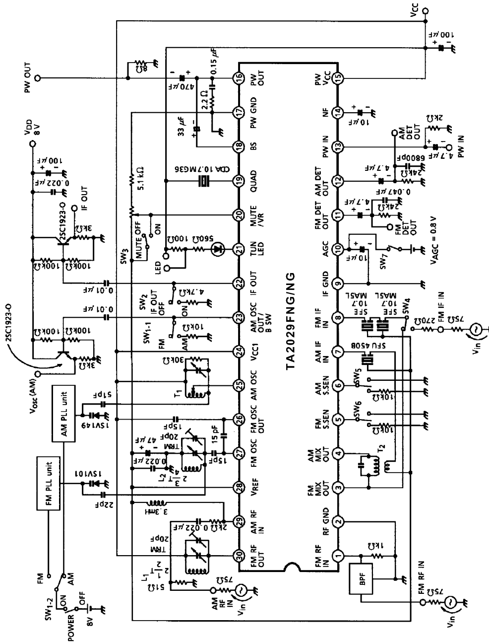
TEST CIRCUIT 1
