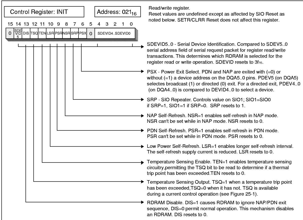
Figure 22-1 Control Registers (1/6)
