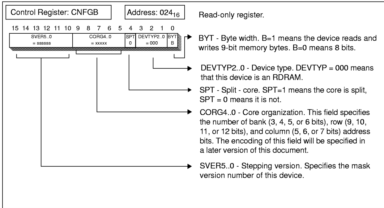
Figure 22-1 Control Registers (2/6)
