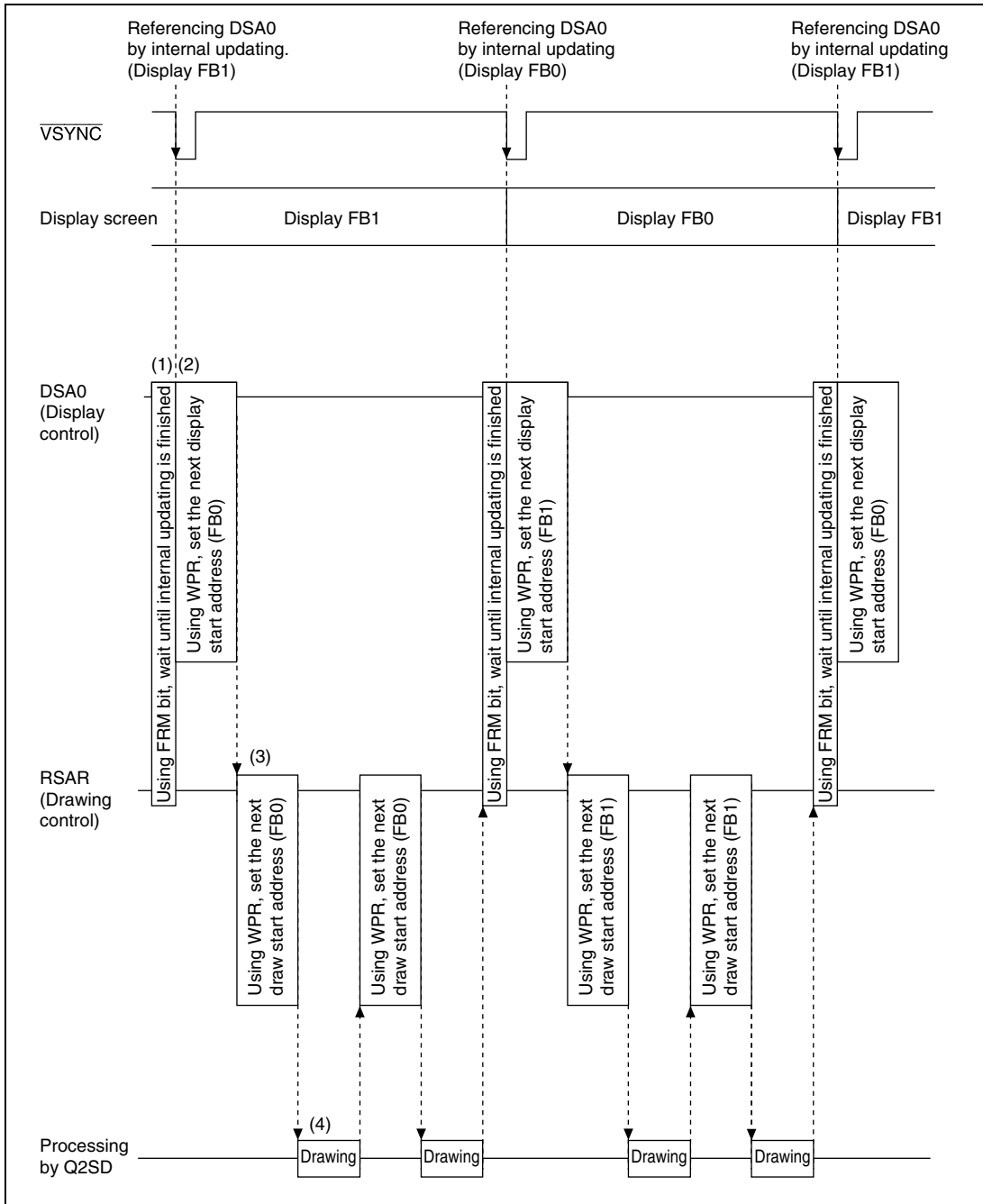
Figure H.1 Display/Drawing Control Timing Chart (DBF = 0)
